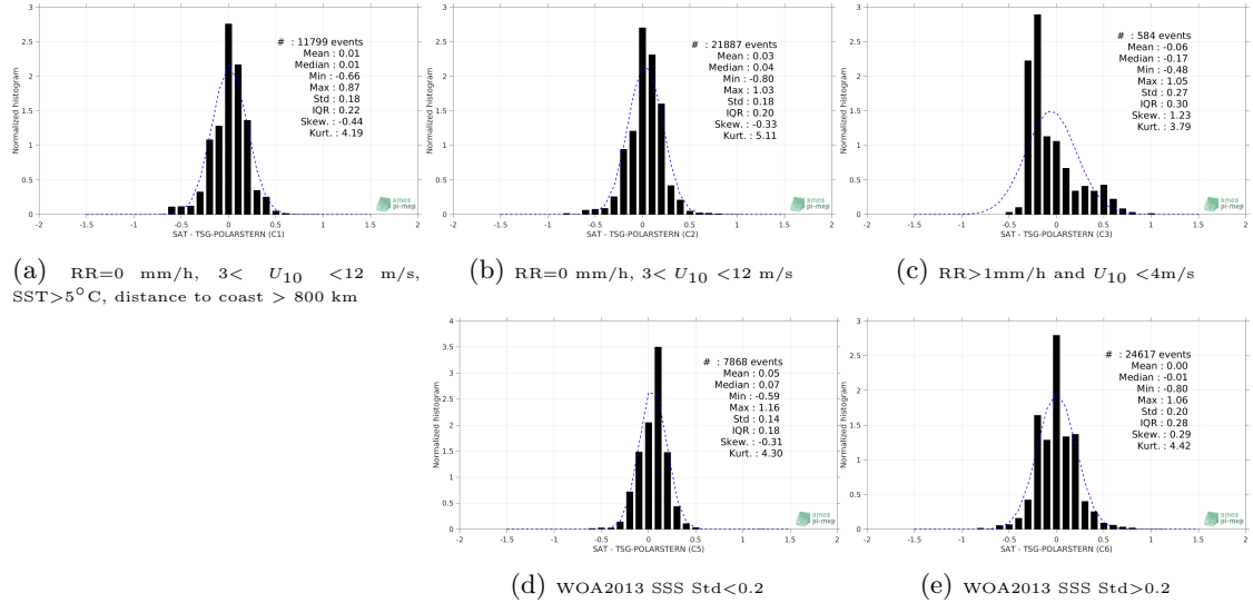
Figure 13: Normalized histogram of \Delta SSS (SMOS-L3-CATDS-CPDC-V317-MONTHLY-25KM - TSG-POLARSTERN) for 5 different subdatasets corresponding to: RR=0 mm/h, 3 < U_{10} < 12 m/s, SST >5^\circ C, distance to coast > 800 km (a), RR=0 mm/h, 3 < U_{10} < 12 m/s (b), RR >1 mm/h and U_{10} < 4 m/s (c), WOA2013 SSS Std <0.2 (d), WOA2013 SSS Std >0.2 (e).
