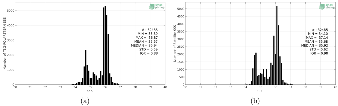
Figure 2: Histograms of SSS from TSG-POLARSTERN (a) and SMOS-L3-CATDS-CPDC-V317-MONTHLY-25KM (b) considering all match-up pairs per bins of 0.1 over the Equatorial Ocean 10N-10S Pi-MEP region and for the full satellite product period.
