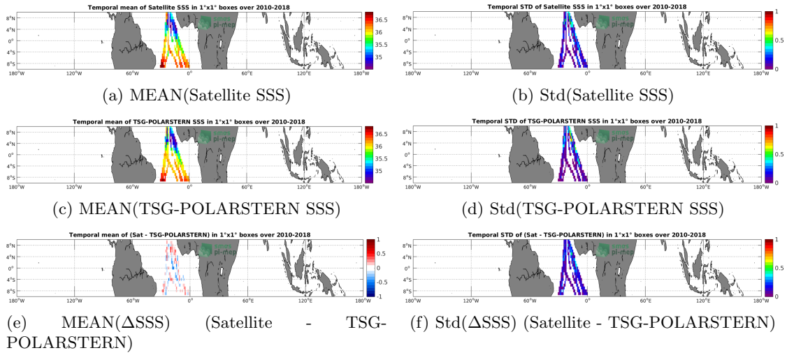
Figure 6: Temporal mean (left) and Std (right) of SSS from SMOS-L3-CATDS-CPDC-V317-MONTHLY-25KM (top), TSG-POLARSTERN (middle), and of \Delta SSS (Satellite - TSG-POLARSTERN). Only match-up pairs are used to generate these maps.
