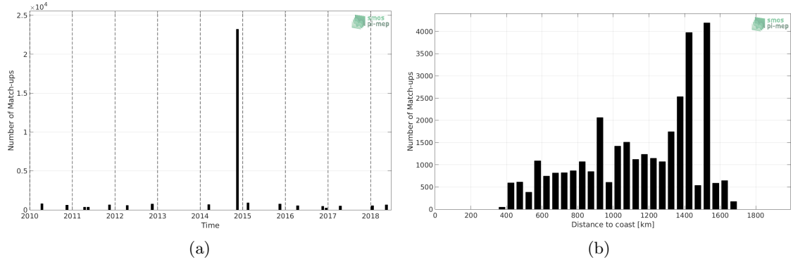
Figure 1: Number of match-ups between TSG-POLARSTERN and SMOS-L3-CATDS-CPDC-V317-MONTHLY-25KM SSS as a function of time (a) and as function of the distance to coast (b) over the Equatorial Ocean 10N-10S Pi-MEP region and for the full satellite product period.
