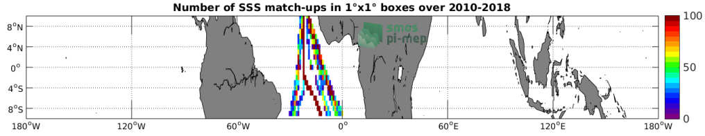
Figure 4: Number of SSS match-ups between TSG-POLARSTERN SSS and the SMOS-L3-CATDS-CPDC-V317-MONTHLY-25KM SSS product for the Equatorial Ocean 10N-10S Pi-MEP region over 1^\circ \times 1^\circ boxes and for the full satellite product period.
