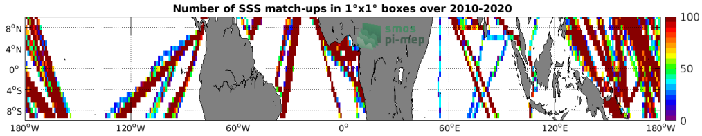
Figure 4: Number of SSS match-ups between TSG (LEGOS-DM) SSS and the SMOS SSS L3 v317 - Monthly - 25 km (CATDS-CPDC) SSS product for the Equatorial Ocean 10N-10S Pi-MEP region over 1^\circ \times 1^\circ boxes and for the full satellite product period.
