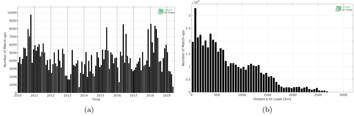
Figure 1: Number of match-ups between TSG (LEGOS-DM) and SMOS SSS L3 v317 - Monthly - 25 km (CATDS-CPDC) SSS as a function of time (a) and as function of the distance to coast (b) over the Equatorial Ocean 10N-10S Pi-MEP region and for the full satellite product period.
