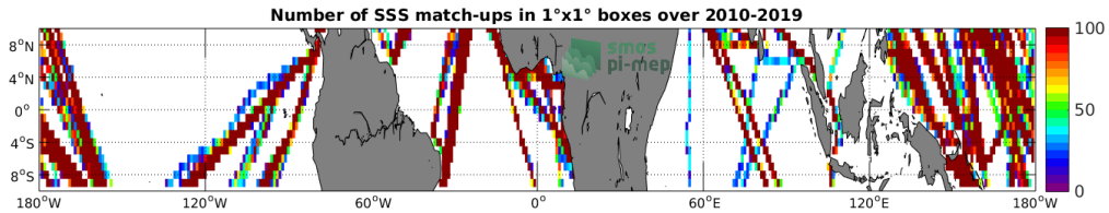
Figure 4: Number of SSS match-ups between TSG (LEGOS-DM) SSS and the SMOS SSS L3 v317 - Monthly - 25 km (CATDS-CPDC) SSS product for the Equatorial Ocean 10N-10S Pi-MEP region over 1°x1° boxes and for the full satellite product period.
