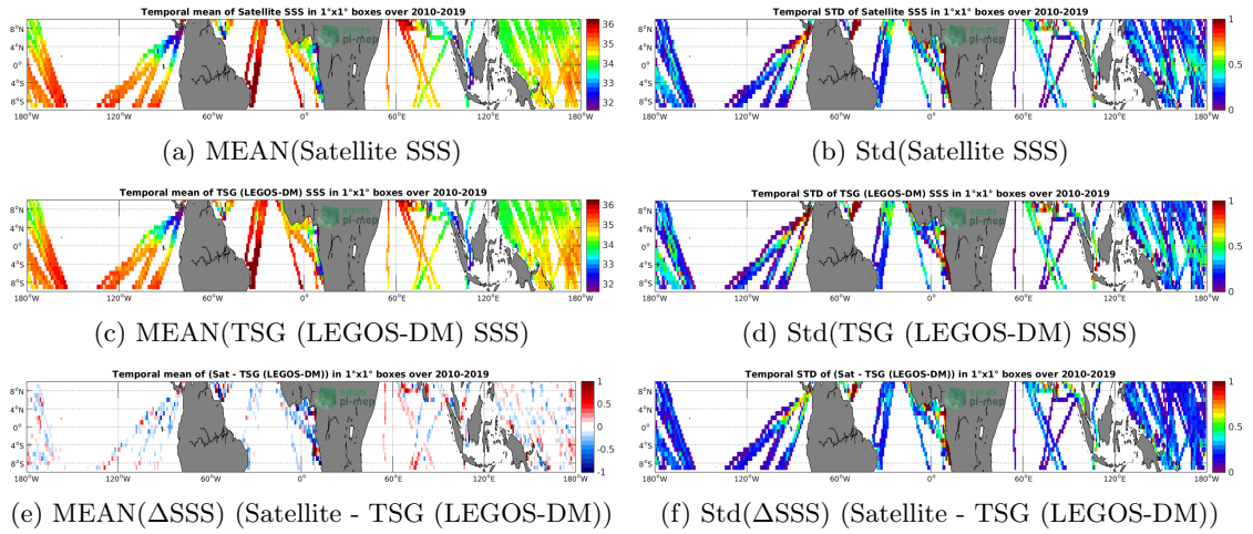
Figure 6: Temporal mean (left) and Std (right) of SSS from SMOS SSS L3 v317 - Monthly - 25 km (CATDS-CPDC) (top), TSG (LEGOS-DM) (middle), and of \Delta SSS (Satellite - TSG (LEGOS-DM)). Only match-up pairs are used to generate these maps.
