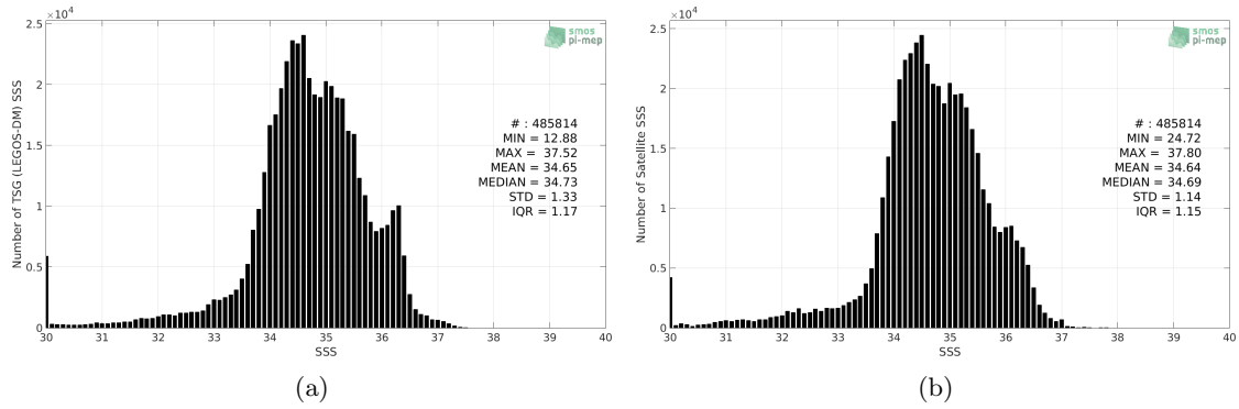
Figure 2: Histograms of SSS from TSG (LEGOS-DM) (a) and SMOS SSS L3 v317 - Monthly - 25 km (CATDS-CPDC) (b) considering all match-up pairs per bins of 0.1 over the Equatorial Ocean 10N-10S Pi-MEP region and for the full satellite product period.
