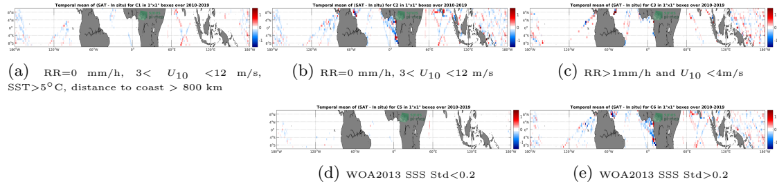
Figure 12: Temporal mean gridded over spatial boxes of size 1^{\circ}\times 1^{\circ} of \Delta\text{SSS} (SMOS SSS L3 v317 - Monthly - 25 km (CATDS-CPDC) - TSG (LEGOS-DM)) for 5 different subdatasets corresponding to: \text{RR}=0 mm/h, 3 < U_{10} < 12 m/s, SST > 5^{\circ}\text{C} , distance to coast > 800 km (a), \text{RR}=0 mm/h, 3 < U_{10} < 12 m/s (b), \text{RR} > 1 mm/h and U_{10} < 4 m/s (c), WOA2013 SSS Std < 0.2 (d), WOA2013 SSS Std > 0.2 (e).
