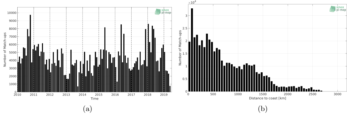
Figure 1: Number of match-ups between TSG-LEGOS-DM and SMOS L3 v317 - Monthly - 25 km (CATDS-CPDC) SSS as a function of time (a) and as function of the distance to coast (b) over the Equatorial Ocean 10N-10S Pi-MEP region and for the full satellite product period.
