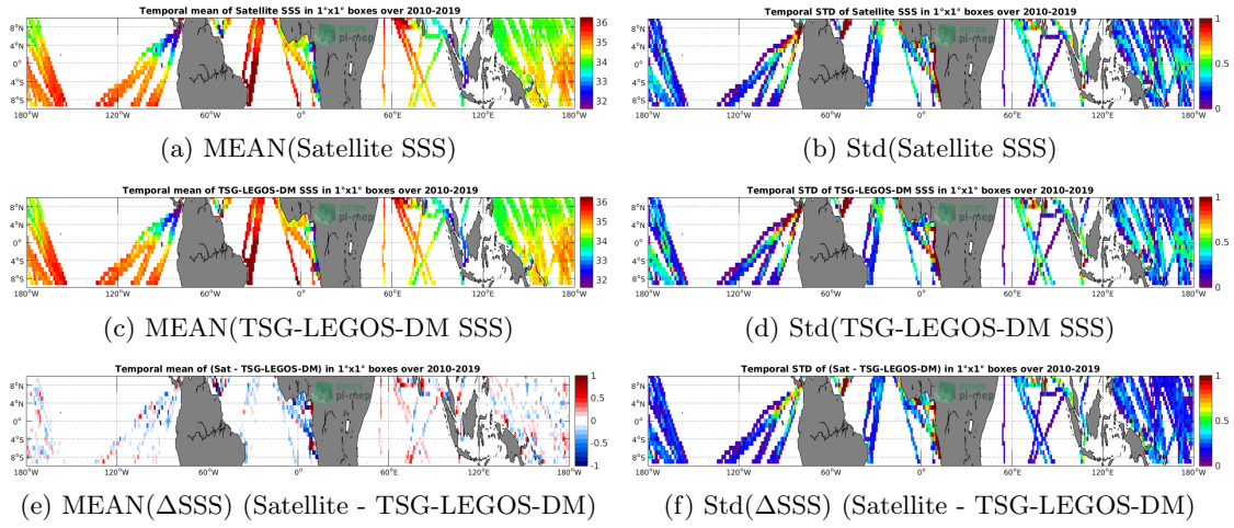
Figure 6: Temporal mean (left) and Std (right) of SSS from SMOS L3 v317 - Monthly - 25 km (CATDS-CPDC) (top), TSG-LEGOS-DM (middle), and of \Delta SSS (Satellite - TSG-LEGOS-DM). Only match-up pairs are used to generate these maps.
