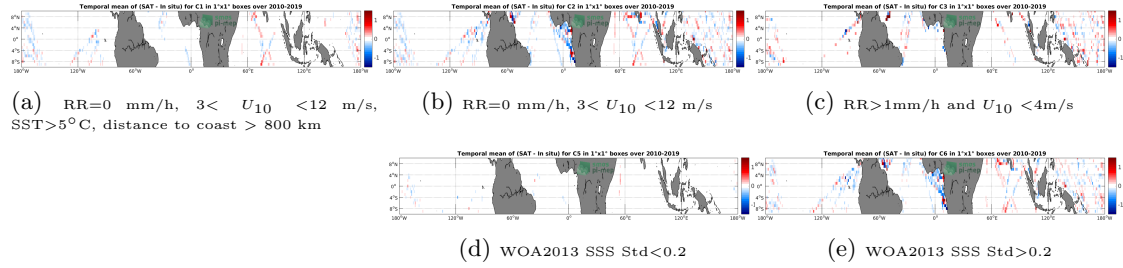
Figure 12: Temporal mean gridded over spatial boxes of size 1^\circ \times 1^\circ of \Delta SSS (SMOS L3 v317 - Monthly - 25 km (CATDS-CPDC) - TSG-LEGOS-DM) for 5 different subdatasets corresponding to: RR=0 mm/h, 3 < U_{10} < 12 m/s, SST > 5^\circ C , distance to coast > 800 km (a), RR=0 mm/h, 3 < U_{10} < 12 m/s (b), RR > 1 mm/h and U_{10} < 4 m/s (c), WOA2013 SSS Std < 0.2 (d), WOA2013 SSS Std > 0.2 (e).
