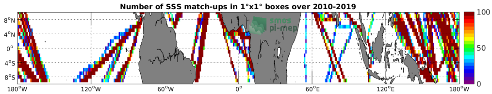
Figure 4: Number of SSS match-ups between TSG-LEGOS-DM SSS and the SMOS L3 v317 - Monthly - 25 km (CATDS-CPDC) SSS product for the Equatorial Ocean 10N-10S Pi-MEP region over 1^\circ \times 1^\circ boxes and for the full satellite product period.
