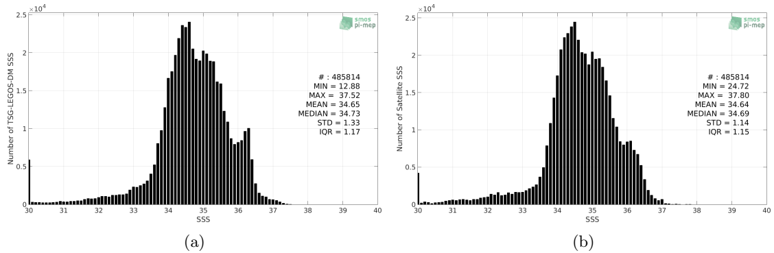
Figure 2: Histograms of SSS from TSG-LEGOS-DM (a) and SMOS L3 v317 - Monthly - 25 km (CATDS-CPDC) (b) considering all match-up pairs per bins of 0.1 over the Equatorial Ocean 10N-10S Pi-MEP region and for the full satellite product period.
