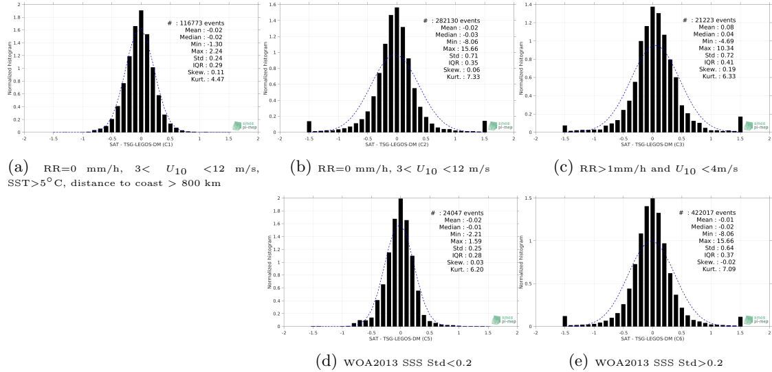
Figure 13: Normalized histogram of \Delta SSS (SMOS-L3-CATDS-CPDC-V317-MONTHLY-25KM - TSG-LEGOS-DM) for 5 different subdatasets corresponding to: RR=0 mm/h, 3 < U_{10} < 12 m/s, SST >5^\circ C, distance to coast > 800 km (a), RR=0 mm/h, 3 < U_{10} < 12 m/s (b), RR >1 mm/h and U_{10} < 4 m/s (c), WOA2013 SSS Std <0.2 (d), WOA2013 SSS Std >0.2 (e).
