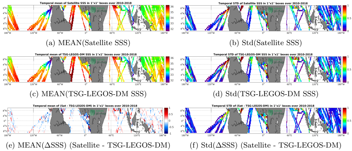
Figure 6: Temporal mean (left) and Std (right) of SSS from SMOS-L3-CATDS-CPDC-V317-MONTHLY-25KM (top), TSG-LEGOS-DM (middle), and of \Delta SSS (Satellite - TSG-LEGOS-DM). Only match-up pairs are used to generate these maps.
