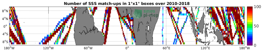
Figure 4: Number of SSS match-ups between TSG-LEGOS-DM SSS and the SMOS-L3-CATDS-CPDC-V317-MONTHLY-25KM SSS product for the Equatorial Ocean 10N-10S Pi-MEP region over 1°x1° boxes and for the full satellite product period.
