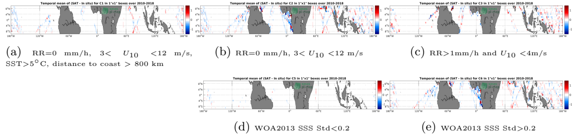
Figure 12: Temporal mean gridded over spatial boxes of size 1^\circ \times 1^\circ of \Delta SSS (SMOS-L3-CATDS-CPDC-V317-MONTHLY-25KM - TSG-LEGOS-DM) for 5 different subdatasets corresponding to:RR=0 mm/h, 3 < U_{10} < 12 m/s, SST >5^\circ C, distance to coast > 800 km (a), RR=0 mm/h, 3 < U_{10} < 12 m/s (b), RR >1 mm/h and U_{10} < 4 m/s (c), WOA2013 SSS Std <0.2 (d), WOA2013 SSS Std >0.2 (e).
