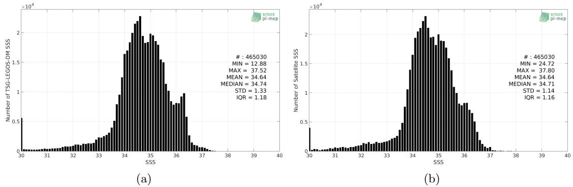
Figure 2: Histograms of SSS from TSG-LEGOS-DM (a) and SMOS-L3-CATDS-CPDC-V317-MONTHLY-25KM (b) considering all match-up pairs per bins of 0.1 over the Equatorial Ocean 10N-10S Pi-MEP region and for the full satellite product period.
