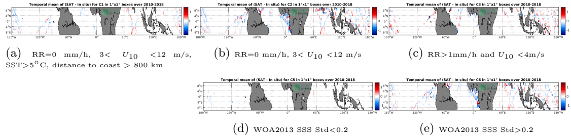
Figure 12: Temporal mean gridded over spatial boxes of size 1^\circ \times 1^\circ of \Delta SSS (SMOS-L3-CATDS-CPDC-V317-MONTHLY-25KM - TSG-LEGOS-DM) for 5 different subdatasets corresponding to:RR=0 mm/h, 3 < U_{10} < 12 m/s, SST >5^\circ C, distance to coast > 800 km (a), RR=0 mm/h, 3 < U_{10} < 12 m/s (b), RR >1 mm/h and U_{10} < 4 m/s (c), WOA2013 SSS Std <0.2 (d), WOA2013 SSS Std >0.2 (e).
