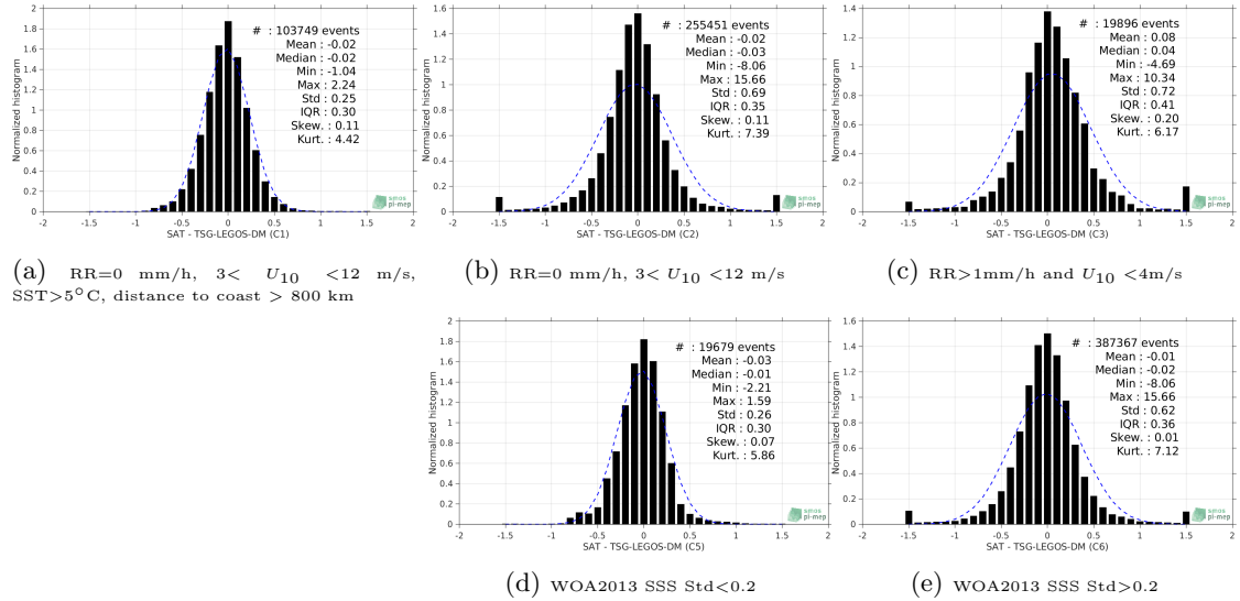
Figure 13: Normalized histogram of \Delta SSS (SMOS-L3-CATDS-CPDC-V317-MONTHLY-25KM - TSG-LEGOS-DM) for 5 different subdatasets corresponding to: RR=0 mm/h, 3 < U_{10} < 12 m/s, SST >5^\circ C, distance to coast > 800 km (a), RR=0 mm/h, 3 < U_{10} < 12 m/s (b), RR >1 mm/h and U_{10} < 4 m/s (c), WOA2013 SSS Std <0.2 (d), WOA2013 SSS Std >0.2 (e).
