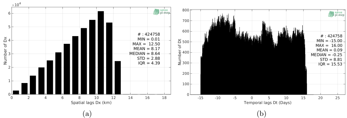
Figure 5: Histograms of the spatial (a) and temporal (b) lags between the time of the TSG-LEGOS-DM measurements and the date of the corresponding SMOS-L3-CATDS-CPDC-V317-MONTHLY-25KM SSS product.
