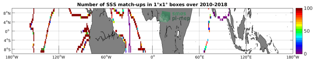
Figure 4: Number of SSS match-ups between TSG (GOSUD-Sailing-ship) SSS and the SMOS SSS L3 v317 - Monthly - 25 km (CATDS-CPDC) SSS product for the Equatorial Ocean 10N-10S Pi-MEP region over 1^\circ \times 1^\circ boxes and for the full satellite product period.
