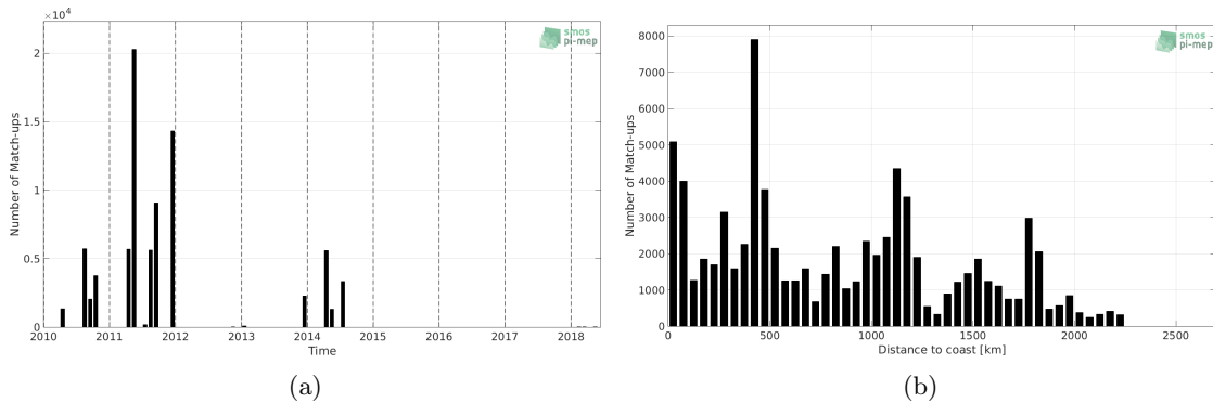
Figure 1: Number of match-ups between TSG (GOSUD-Sailing-ship) and SMOS SSS L3 v317 - Monthly - 25 km (CATDS-CPDC) SSS as a function of time (a) and as function of the distance to coast (b) over the Equatorial Ocean 10N-10S Pi-MEP region and for the full satellite product period.
