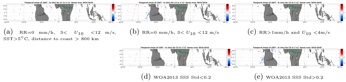
Figure 12: Temporal mean gridded over spatial boxes of size 1^\circ \times 1^\circ of \Delta SSS (SMOS SSS L3 v317 - Monthly - 25 km (CATDS-CPDC) - TSG (GOSUD-Sailing-ship)) for 5 different subdatasets corresponding to:RR=0 mm/h, 3 < U_{10} < 12 m/s, SST >5^\circ\text{C} , distance to coast > 800 km (a), RR=0 mm/h, 3 < U_{10} < 12 m/s (b), RR >1 mm/h and U_{10} < 4 m/s (c), WOA2013 SSS Std <0.2 (d), WOA2013 SSS Std >0.2 (e).
