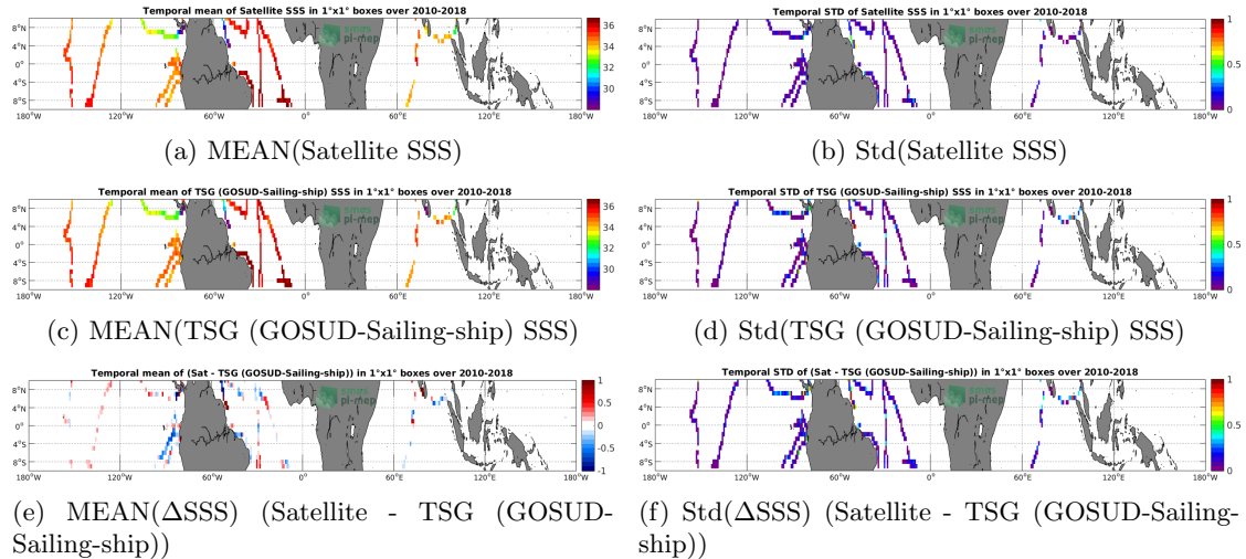
Figure 6: Temporal mean (left) and Std (right) of SSS from SMOS SSS L3 v317 - Monthly - 25 km (CATDS-CPDC) (top), TSG (GOSUD-Sailing-ship) (middle), and of \Delta SSS (Satellite - TSG (GOSUD-Sailing-ship)). Only match-up pairs are used to generate these maps.
