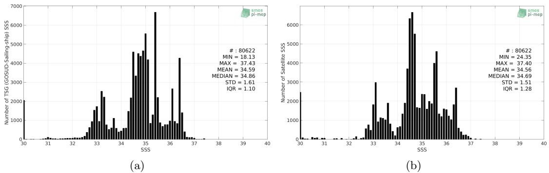
Figure 2: Histograms of SSS from TSG (GOSUD-Sailing-ship) (a) and SMOS SSS L3 v317 - Monthly - 25 km (CATDS-CPDC) (b) considering all match-up pairs per bins of 0.1 over the Equatorial Ocean 10N-10S Pi-MEP region and for the full satellite product period.
