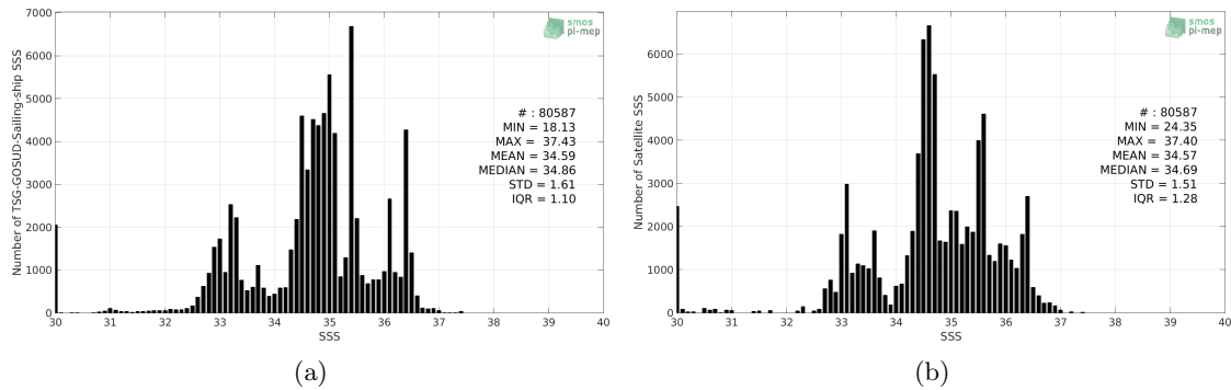
Figure 2: Histograms of SSS from TSG-GOSUD-Sailing-ship (a) and SMOS L3 v317 - Monthly - 25 km (CATDS-CPDC) (b) considering all match-up pairs per bins of 0.1 over the Equatorial Ocean 10N-10S Pi-MEP region and for the full satellite product period.
