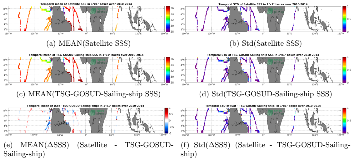
Figure 6: Temporal mean (left) and Std (right) of SSS from SMOS L3 v317 - Monthly - 25 km (CATDS-CPDC) (top), TSG-GOSUD-Sailing-ship (middle), and of \Delta SSS (Satellite - TSG-GOSUD-Sailing-ship). Only match-up pairs are used to generate these maps.
