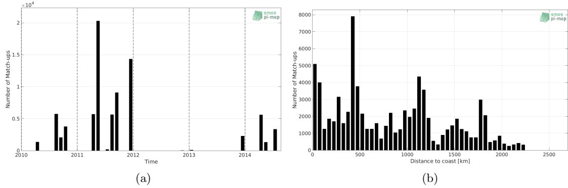
Figure 1: Number of match-ups between TSG-GOSUD-Sailing-ship and SMOS L3 v317 - Monthly - 25 km (CATDS-CPDC) SSS as a function of time (a) and as function of the distance to coast (b) over the Equatorial Ocean 10N-10S Pi-MEP region and for the full satellite product period.
