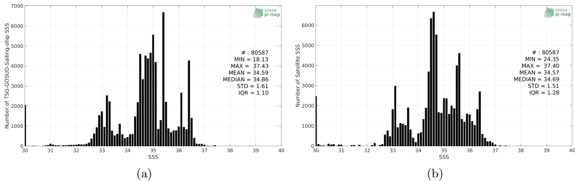
Figure 2: Histograms of SSS from TSG-GOSUD-Sailing-ship (a) and SMOS-L3-CATDS-CPDC-V317-MONTHLY-25KM (b) considering all match-up pairs per bins of 0.1 over the Equatorial Ocean 10N-10S Pi-MEP region and for the full satellite product period.
