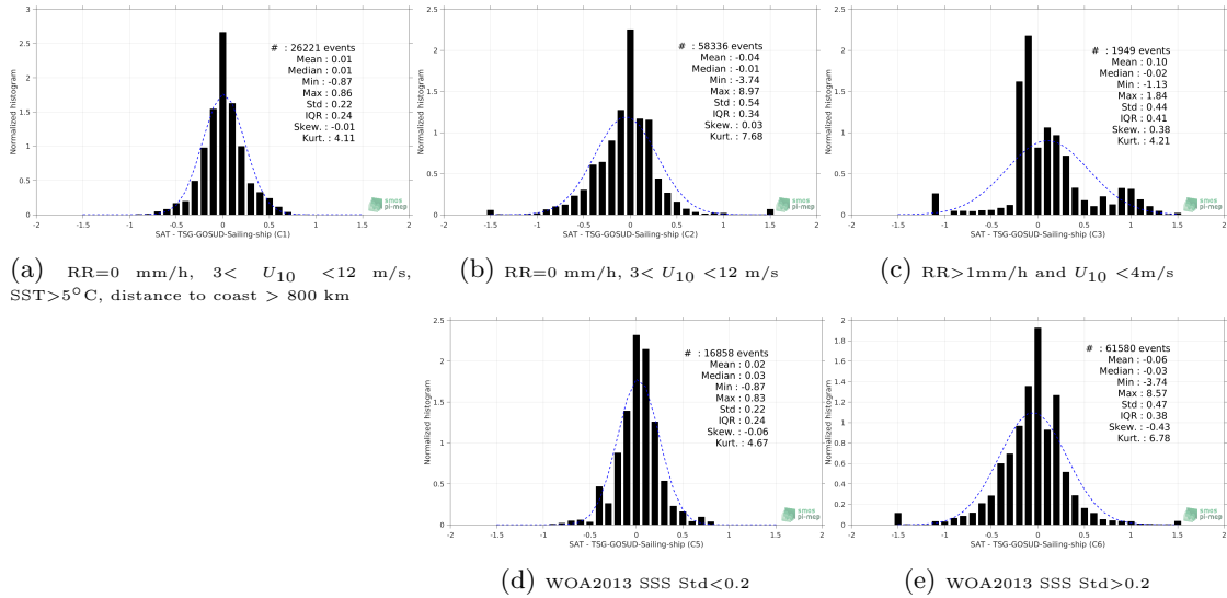
Figure 13: Normalized histogram of \Delta SSS (SMOS-L3-CATDS-CPDC-V317-MONTHLY-25KM - TSG-GOSUD-Sailing-ship) for 5 different subdatasets corresponding to: RR=0 mm/h, 3 < U_{10} < 12 m/s, SST> 5^\circ\text{C} , distance to coast > 800 km (a), RR=0 mm/h, 3 < U_{10} < 12 m/s (b), RR>1mm/h and U_{10} < 4 m/s (c), WOA2013 SSS Std<0.2 (d), WOA2013 SSS Std>0.2 (e).
