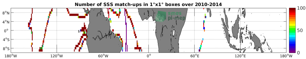
Figure 4: Number of SSS match-ups between TSG-GOSUD-Sailing-ship SSS and the SMOS-L3-CATDS-CPDC-V317-MONTHLY-25KM SSS product for the Equatorial Ocean 10N-10S Pi-MEP region over 1°x1° boxes and for the full satellite product period.
