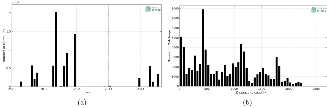
Figure 1: Number of match-ups between TSG-GOSUD-Sailing-ship and SMOS-L3-CATDS-CPDC-V317-MONTHLY-25KM SSS as a function of time (a) and as function of the distance to coast (b) over the Equatorial Ocean 10N-10S Pi-MEP region and for the full satellite product period.
