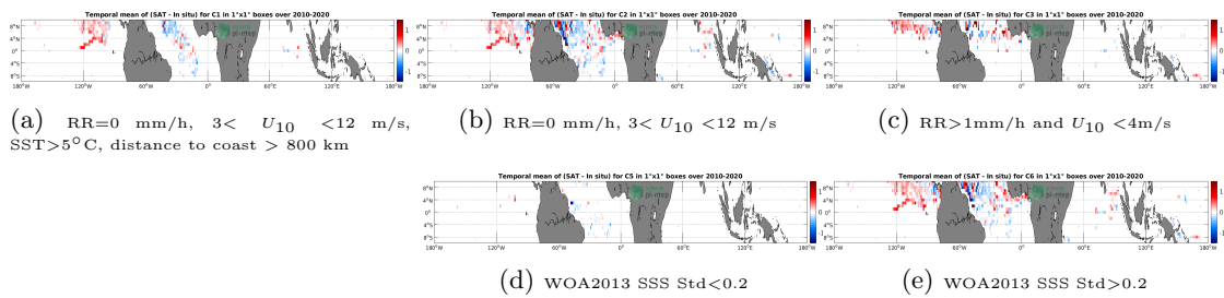
Figure 11: Temporal mean gridded over spatial boxes of size 1°x1° of \Delta SSS (SMOS SSS L3 v317 - Monthly - 25 km (CATDS-CPDC) - Surface drifters) for 5 different subdatasets corresponding to: RR=0 mm/h, 3 < U_{10} < 12 m/s, SST>5°C, distance to coast > 800 km (a), RR=0 mm/h, 3 < U_{10} < 12 m/s (b), RR>1mm/h and U_{10} < 4 m/s (c), WOA2013 SSS Std<0.2 (d), WOA2013 SSS Std>0.2 (e).
