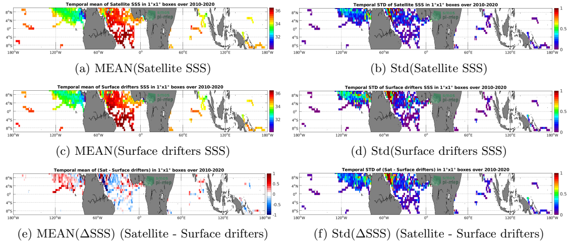
Figure 5: Temporal mean (left) and Std (right) of SSS from SMOS SSS L3 v317 - Monthly - 25 km (CATDS-CPDC) (top), Surface drifters (middle), and of \Delta SSS (Satellite - Surface drifters). Only match-up pairs are used to generate these maps.
