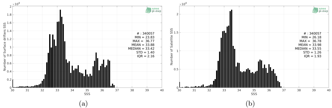
Figure 2: Histograms of SSS from Surface drifters (a) and SMOS SSS L3 v317 - Monthly - 25 km (CATDS-CPDC) (b) considering all match-up pairs per bins of 0.1 over the Equatorial Ocean 10N-10S Pi-MEP region and for the full satellite product period.
