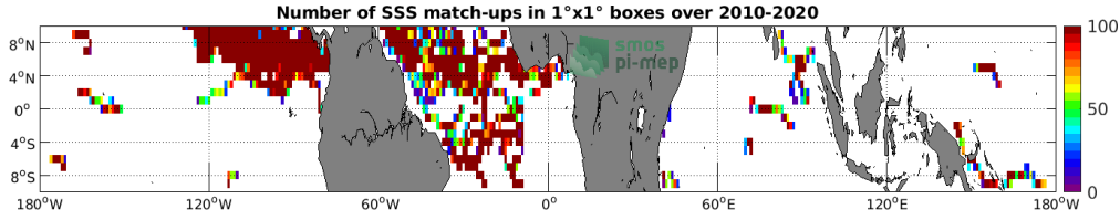
Figure 3: Number of SSS match-ups between Surface drifters SSS and the SMOS SSS L3 v317 - Monthly - 25 km (CATDS-CPDC) SSS product for the Equatorial Ocean 10N-10S Pi-MEP region over 1^\circ \times 1^\circ boxes and for the full satellite product period.
