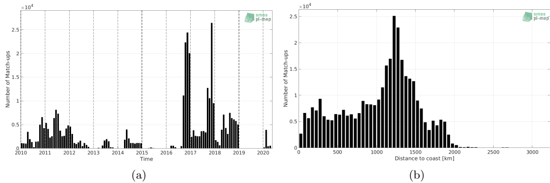
Figure 1: Number of match-ups between Surface drifters and SMOS SSS L3 v317 - Monthly - 25 km (CATDS-CPDC) SSS as a function of time (a) and as function of the distance to coast (b) over the Equatorial Ocean 10N-10S Pi-MEP region and for the full satellite product period.
