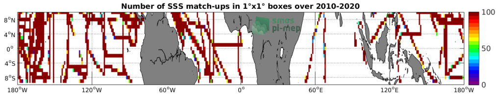
Figure 4: Number of SSS match-ups between TSG-SAMOS SSS and the SMOS L3 v317 - 10 Days - 25 km (CATDS-CPDC) SSS product for the Equatorial Ocean 10N-10S Pi-MEP region over 1°x1° boxes and for the full satellite product period.
