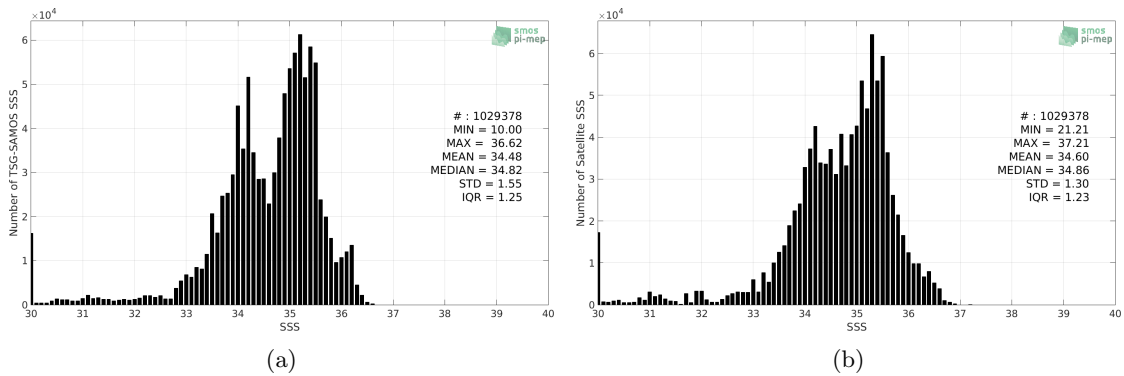
Figure 2: Histograms of SSS from TSG-SAMOS (a) and SMOS L3 v317 - 10 Days - 25 km (CATDS-CPDC) (b) considering all match-up pairs per bins of 0.1 over the Equatorial Ocean 10N-10S Pi-MEP region and for the full satellite product period.
