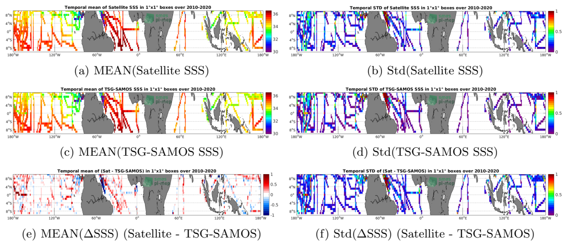
Figure 6: Temporal mean (left) and Std (right) of SSS from SMOS L3 v317 - 10 Days - 25 km (CATDS-CPDC) (top), TSG-SAMOS (middle), and of \Delta SSS (Satellite - TSG-SAMOS). Only match-up pairs are used to generate these maps.
