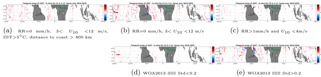
Figure 12: Temporal mean gridded over spatial boxes of size 1^\circ \times 1^\circ of \Delta SSS (SMOS L3 v317 - 10 Days - 25 km (CATDS-CPDC) - TSG-SAMOS) for 5 different subdatasets corresponding to: RR=0 mm/h, 3 < U_{10} < 12 m/s, SST >5^\circ\text{C} , distance to coast > 800 km (a), RR=0 mm/h, 3 < U_{10} < 12 m/s (b), RR >1 mm/h and U_{10} < 4 m/s (c), WOA2013 SSS Std <0.2 (d), WOA2013 SSS Std >0.2 (e).
