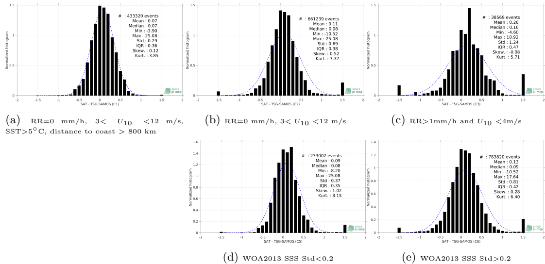
Figure 13: Normalized histogram of \Delta SSS (SMOS L3 v317 - 10 Days - 25 km (CATDS-CPDC) - TSG-SAMOS) for 5 different subdatasets corresponding to: RR=0 mm/h, 3 < U_{10} < 12 m/s, SST >5^\circ\text{C} , distance to coast > 800 km (a), RR=0 mm/h, 3 < U_{10} < 12 m/s (b), RR >1 mm/h and U_{10} < 4 m/s (c), WOA2013 SSS Std <0.2 (d), WOA2013 SSS Std >0.2 (e).
