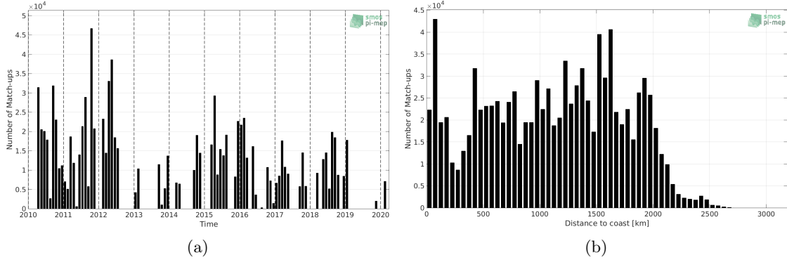
Figure 1: Number of match-ups between TSG-SAMOS and SMOS L3 v317 - 10 Days - 25 km (CATDS-CPDC) SSS as a function of time (a) and as function of the distance to coast (b) over the Equatorial Ocean 10N-10S Pi-MEP region and for the full satellite product period.
