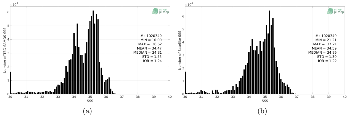
Figure 2: Histograms of SSS from TSG-SAMOS (a) and SMOS-L3-CATDS-CPDC-V317-10DAYS-25KM (b) considering all match-up pairs per bins of 0.1 over the Equatorial Ocean 10N-10S Pi-MEP region and for the full satellite product period.
