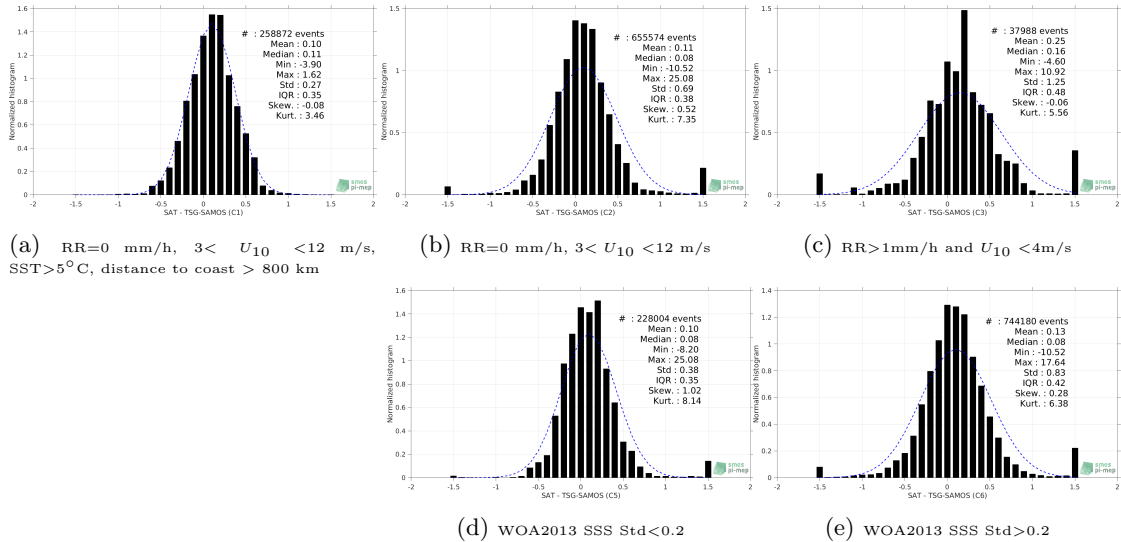
Figure 13: Normalized histogram of \Delta SSS (SMOS-L3-CATDS-CPDC-V317-10DAYS-25KM - TSG-SAMOS) for 5 different subdatasets corresponding to: RR=0 mm/h, 3 < U_{10} < 12 m/s, SST >5^\circ C, distance to coast > 800 km (a), RR=0 mm/h, 3 < U_{10} < 12 m/s (b), RR >1 mm/h and U_{10} < 4 m/s (c), WOA2013 SSS Std <0.2 (d), WOA2013 SSS Std >0.2 (e).
