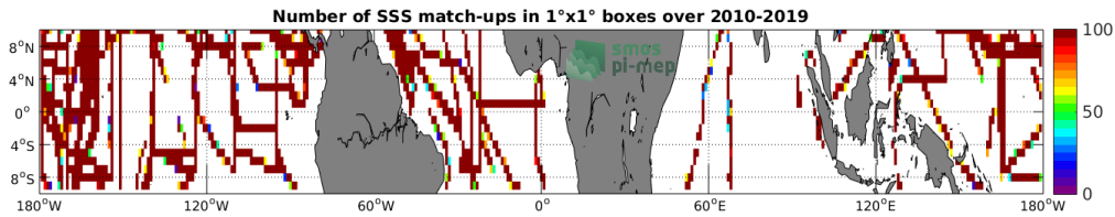
Figure 4: Number of SSS match-ups between TSG-SAMOS SSS and the SMOS-L3-CATDS-CPDC-V317-10DAYS-25KM SSS product for the Equatorial Ocean 10N-10S Pi-MEP region over 1^\circ \times 1^\circ boxes and for the full satellite product period.
