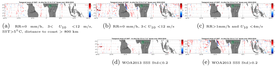
Figure 12: Temporal mean gridded over spatial boxes of size 1^\circ \times 1^\circ of \Delta SSS (SMOS-L3-CATDS-CPDC-V317-10DAYS-25KM - TSG-SAMOS) for 5 different subdatasets corresponding to:RR=0 mm/h, 3 < U_{10} < 12 m/s, SST >5^\circ C, distance to coast > 800 km (a), RR=0 mm/h, 3 < U_{10} < 12 m/s (b), RR >1 mm/h and U_{10} < 4 m/s (c), WOA2013 SSS Std <0.2 (d), WOA2013 SSS Std >0.2 (e).
