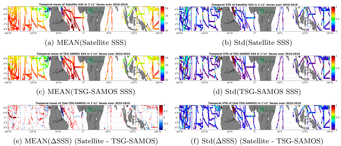
Figure 6: Temporal mean (left) and Std (right) of SSS from SMOS-L3-CATDS-CPDC-V317-10DAYS-25KM (top), TSG-SAMOS (middle), and of \Delta SSS (Satellite - TSG-SAMOS). Only match-up pairs are used to generate these maps.
