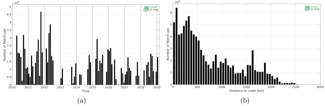
Figure 1: Number of match-ups between TSG-SAMOS and SMOS-L3-CATDS-CPDC-V317-10DAYS-25KM SSS as a function of time (a) and as function of the distance to coast (b) over the Equatorial Ocean 10N-10S Pi-MEP region and for the full satellite product period.
