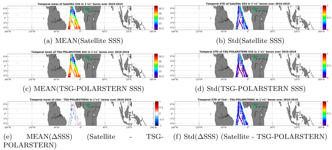
Figure 6: Temporal mean (left) and Std (right) of SSS from SMOS L3 v317 - 10 Days - 25 km (CATDS-CPDC) (top), TSG-POLARSTERN (middle), and of \Delta SSS (Satellite - TSG-POLARSTERN). Only match-up pairs are used to generate these maps.
