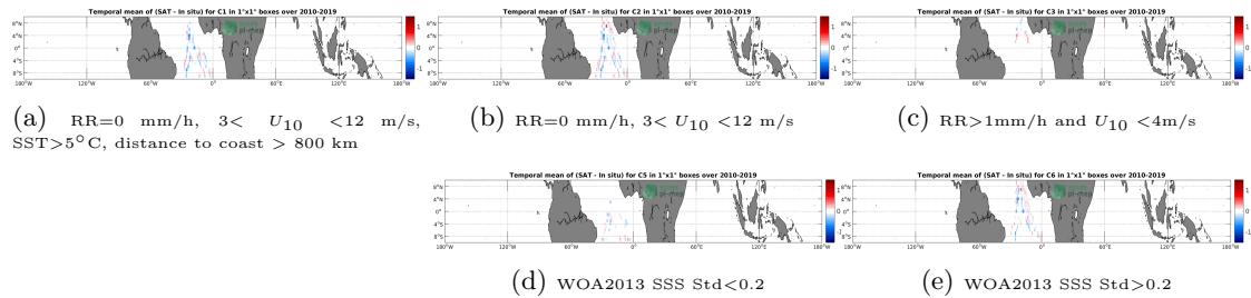
Figure 12: Temporal mean gridded over spatial boxes of size 1^{\circ}\times 1^{\circ} of \Delta\text{SSS} (SMOS L3 v317 - 10 Days - 25 km (CATDS-CPDC) - TSG-POLARSTERN) for 5 different subdatasets corresponding to:RR=0 mm/h, 3 < U_{10} < 12 m/s, SST >5^{\circ}\text{C} , distance to coast > 800 km (a), RR=0 mm/h, 3 < U_{10} < 12 m/s (b), RR >1 mm/h and U_{10} < 4 m/s (c), WOA2013 SSS Std <0.2 (d), WOA2013 SSS Std >0.2 (e).
