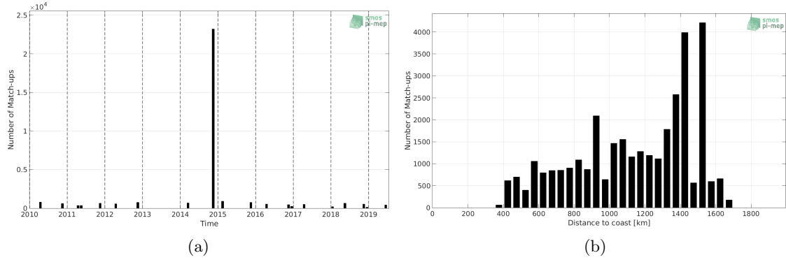
Figure 1: Number of match-ups between TSG-POLARSTERN and SMOS L3 v317 - 10 Days - 25 km (CATDS-CPDC) SSS as a function of time (a) and as function of the distance to coast (b) over the Equatorial Ocean 10N-10S Pi-MEP region and for the full satellite product period.
