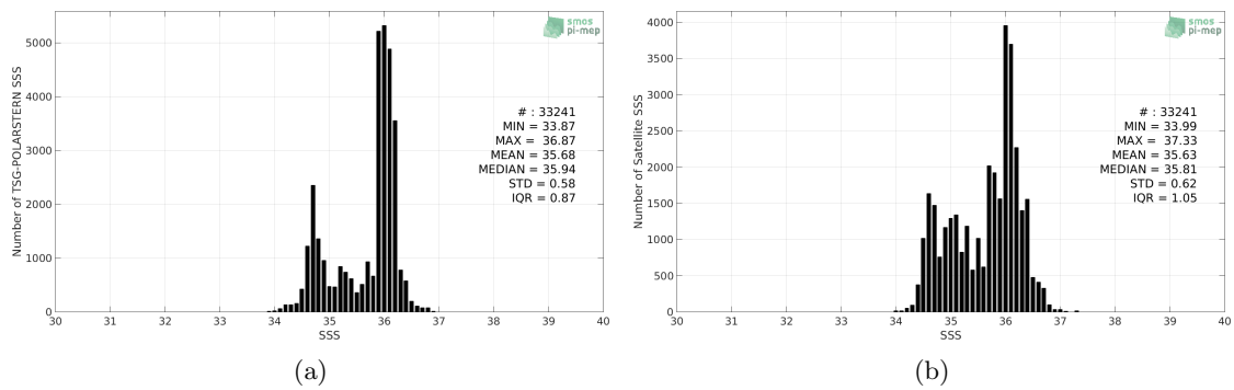
Figure 2: Histograms of SSS from TSG-POLARSTERN (a) and SMOS L3 v317 - 10 Days - 25 km (CATDS-CPDC) (b) considering all match-up pairs per bins of 0.1 over the Equatorial Ocean 10N-10S Pi-MEP region and for the full satellite product period.
