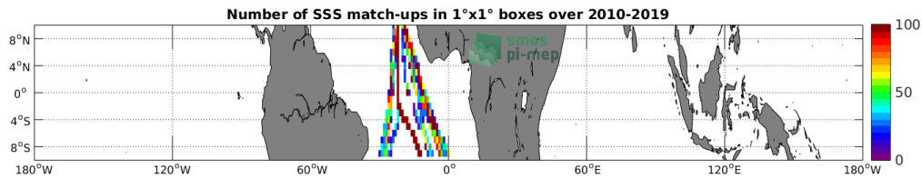
Figure 4: Number of SSS match-ups between TSG-POLARSTERN SSS and the SMOS L3 v317 - 10 Days - 25 km (CATDS-CPDC) SSS product for the Equatorial Ocean 10N-10S Pi-MEP region over 1°x1° boxes and for the full satellite product period.
