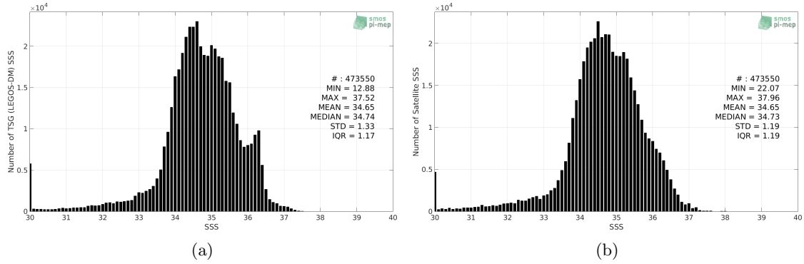
Figure 2: Histograms of SSS from TSG (LEGOS-DM) (a) and SMOS SSS L3 v317 - 10 Days - 25 km (CATDS-CPDC) (b) considering all match-up pairs per bins of 0.1 over the Equatorial Ocean 10N-10S Pi-MEP region and for the full satellite product period.
