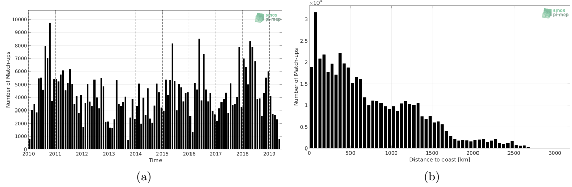
Figure 1: Number of match-ups between TSG (LEGOS-DM) and SMOS SSS L3 v317 - 10 Days - 25 km (CATDS-CPDC) SSS as a function of time (a) and as function of the distance to coast (b) over the Equatorial Ocean 10N-10S Pi-MEP region and for the full satellite product period.
