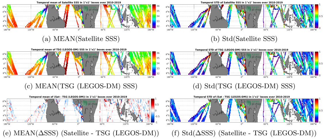
Figure 6: Temporal mean (left) and Std (right) of SSS from SMOS SSS L3 v317 - 10 Days - 25 km (CATDS-CPDC) (top), TSG (LEGOS-DM) (middle), and of \Delta SSS (Satellite - TSG (LEGOS-DM)). Only match-up pairs are used to generate these maps.
