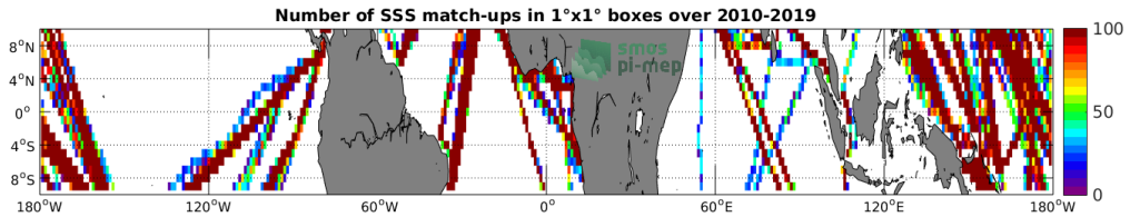
Figure 4: Number of SSS match-ups between TSG (LEGOS-DM) SSS and the SMOS SSS L3 v317 - 10 Days - 25 km (CATDS-CPDC) SSS product for the Equatorial Ocean 10N-10S Pi-MEP region over 1^\circ \times 1^\circ boxes and for the full satellite product period.
