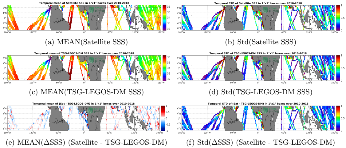
Figure 6: Temporal mean (left) and Std (right) of SSS from SMOS-L3-CATDS-CPDC-V317-10DAYS-25KM (top), TSG-LEGOS-DM (middle), and of \Delta SSS (Satellite - TSG-LEGOS-DM). Only match-up pairs are used to generate these maps.
