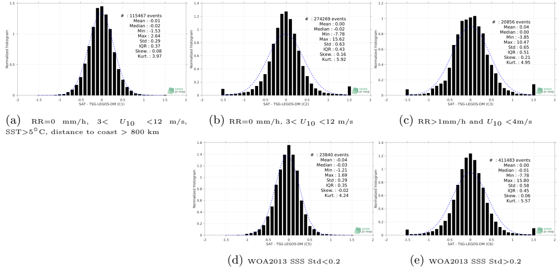
Figure 13: Normalized histogram of \Delta SSS (SMOS-L3-CATDS-CPDC-V317-10DAYS-25KM - TSG-LEGOS-DM) for 5 different subdatasets corresponding to: RR=0 mm/h, 3 < U_{10} < 12 m/s, SST > 5^\circ C , distance to coast > 800 km (a), RR=0 mm/h, 3 < U_{10} < 12 m/s (b), RR > 1 mm/h and U_{10} < 4 m/s (c), WOA2013 SSS Std < 0.2 (d), WOA2013 SSS Std > 0.2 (e).
