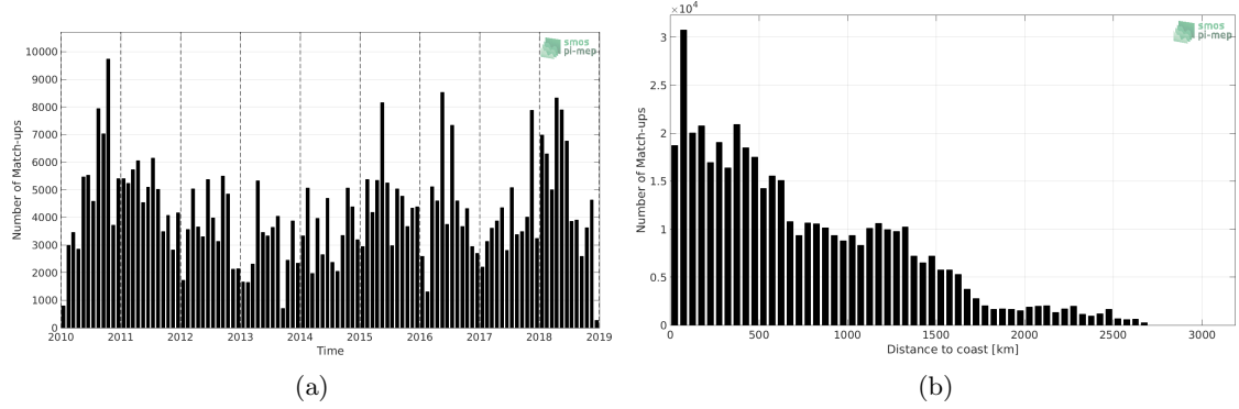
Figure 1: Number of match-ups between TSG-LEGOS-DM and SMOS-L3-CATDS-CPDC-V317-10DAYS-25KM SSS as a function of time (a) and as function of the distance to coast (b) over the Equatorial Ocean 10N-10S Pi-MEP region and for the full satellite product period.
