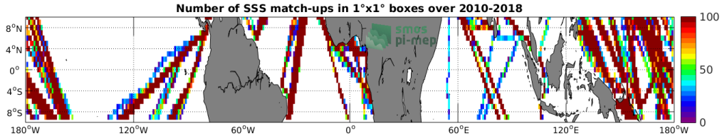
Figure 4: Number of SSS match-ups between TSG-LEGOS-DM SSS and the SMOS-L3-CATDS-CPDC-V317-10DAYS-25KM SSS product for the Equatorial Ocean 10N-10S Pi-MEP region over 1^\circ \times 1^\circ boxes and for the full satellite product period.
