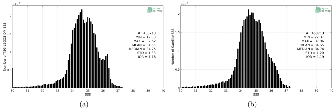
Figure 2: Histograms of SSS from TSG-LEGOS-DM (a) and SMOS-L3-CATDS-CPDC-V317-10DAYS-25KM (b) considering all match-up pairs per bins of 0.1 over the Equatorial Ocean 10N-10S Pi-MEP region and for the full satellite product period.
