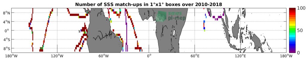
Figure 4: Number of SSS match-ups between TSG (GOSUD-Sailing-ship) SSS and the SMOS SSS L3 v317 - 10 Days - 25 km (CATDS-CPDC) SSS product for the Equatorial Ocean 10N-10S Pi-MEP region over 1^\circ \times 1^\circ boxes and for the full satellite product period.
