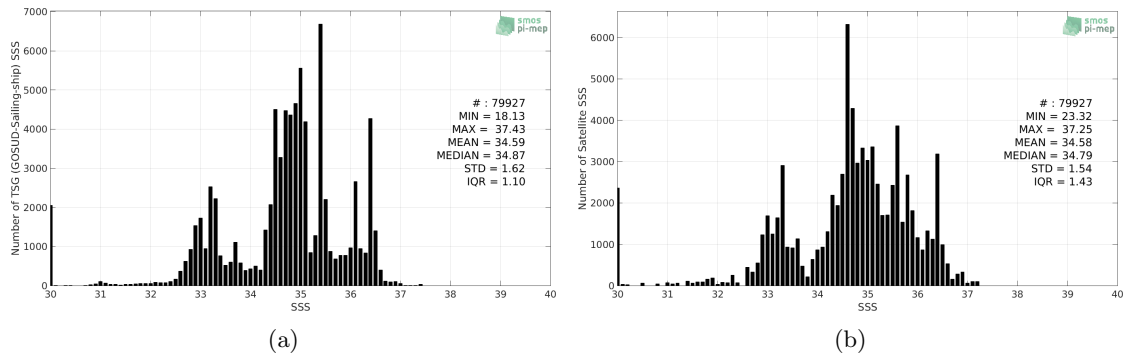
Figure 2: Histograms of SSS from TSG (GOSUD-Sailing-ship) (a) and SMOS SSS L3 v317 - 10 Days - 25 km (CATDS-CPDC) (b) considering all match-up pairs per bins of 0.1 over the Equatorial Ocean 10N-10S Pi-MEP region and for the full satellite product period.
