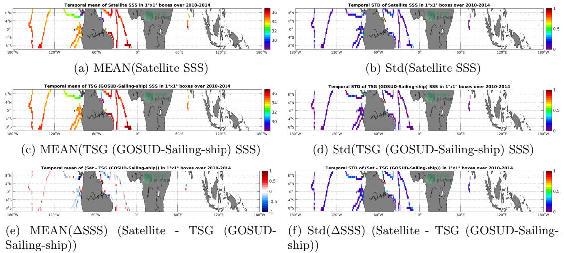
Figure 6: Temporal mean (left) and Std (right) of SSS from SMOS SSS L3 v317 - 10 Days - 25 km (CATDS-CPDC) (top), TSG (GOSUD-Sailing-ship) (middle), and of \Delta SSS (Satellite - TSG (GOSUD-Sailing-ship)). Only match-up pairs are used to generate these maps.
