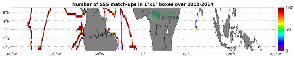
Figure 4: Number of SSS match-ups between TSG (GOSUD-Sailing-ship) SSS and the SMOS SSS L3 v317 - 10 Days - 25 km (CATDS-CPDC) SSS product for the Equatorial Ocean 10N-10S Pi-MEP region over 1°x1° boxes and for the full satellite product period.
