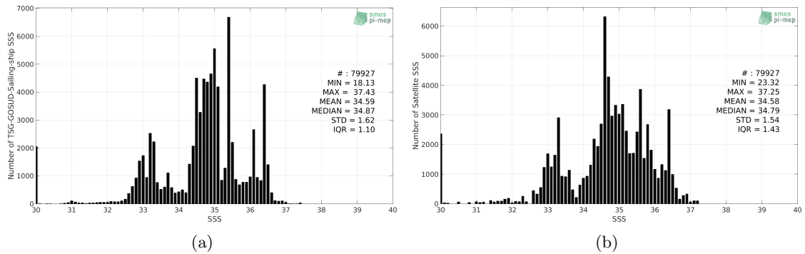
Figure 2: Histograms of SSS from TSG-GOSUD-Sailing-ship (a) and SMOS-L3-CATDS-CPDC-V317-10DAYS-25KM (b) considering all match-up pairs per bins of 0.1 over the Equatorial Ocean 10N-10S Pi-MEP region and for the full satellite product period.
