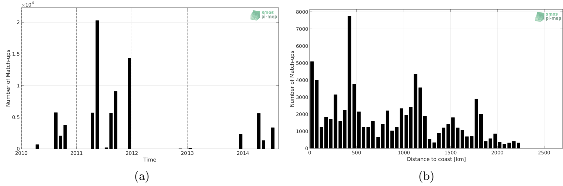
Figure 1: Number of match-ups between TSG-GOSUD-Sailing-ship and SMOS-L3-CATDS-CPDC-V317-10DAYS-25KM SSS as a function of time (a) and as function of the distance to coast (b) over the Equatorial Ocean 10N-10S Pi-MEP region and for the full satellite product period.
