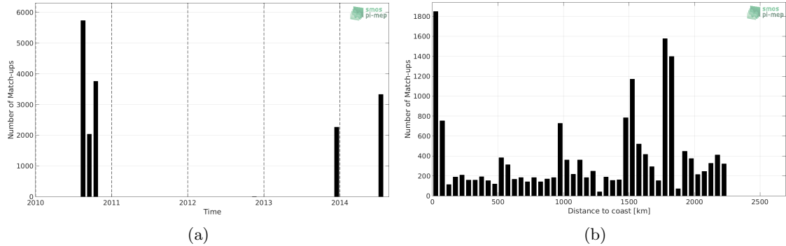
Figure 1: Number of match-ups between TSG-GOSUD-Sailing-ship and SMOS-L3-CATDS-CPDC-V317-10DAYS-25KM SSS as a function of time (a) and as function of the distance to coast (b) over the Equatorial Ocean 10N-10S Pi-MEP region and for the full satellite product period.
