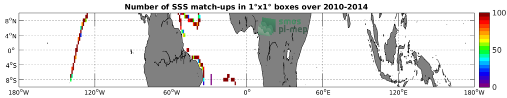
Figure 4: Number of SSS match-ups between TSG-GOSUD-Sailing-ship SSS and the SMOS-L3-CATDS-CPDC-V317-10DAYS-25KM SSS product for the Equatorial Ocean 10N-10S Pi-MEP region over 1°x1° boxes and for the full satellite product period.
