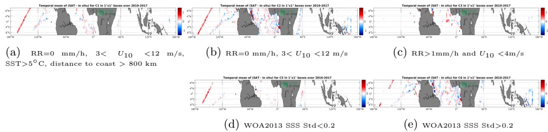
Figure 12: Temporal mean gridded over spatial boxes of size 1^\circ \times 1^\circ of \Delta SSS (SMOS-L3-CATDS-CPDC-V317-10DAYS-25KM - TSG-GOSUD-Research-vessel) for 5 different subdatasets corresponding to: RR=0 mm/h, 3 < U_{10} < 12 m/s, SST > 5^\circ\text{C} , distance to coast > 800 km (a), RR=0 mm/h, 3 < U_{10} < 12 m/s (b), RR > 1\text{mm/h} and U_{10} < 4\text{m/s} (c), WOA2013 SSS Std < 0.2 (d), WOA2013 SSS Std > 0.2 (e).
