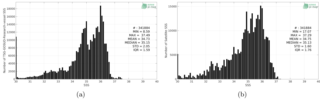
Figure 2: Histograms of SSS from TSG-GOSUD-Research-vessel (a) and SMOS-L3-CATDS-CPDC-V317-10DAYS-25KM (b) considering all match-up pairs per bins of 0.1 over the Equatorial Ocean 10N-10S Pi-MEP region and for the full satellite product period.
