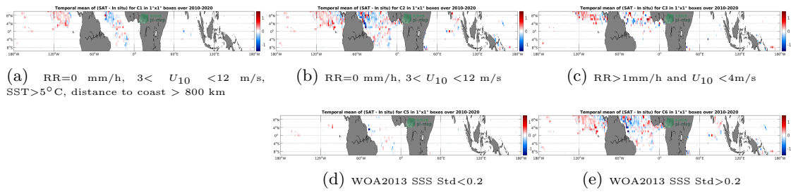
Figure 11: Temporal mean gridded over spatial boxes of size 1°x1° of \Delta SSS (SMOS SSS L3 v317 - 10 Days - 25 km (CATDS-CPDC) - Surface drifters) for 5 different subdatasets corresponding to: RR=0 mm/h, 3 < U_{10} < 12 m/s, SST>5°C, distance to coast > 800 km (a), RR=0 mm/h, 3 < U_{10} < 12 m/s (b), RR>1mm/h and U_{10} < 4m/s (c), WOA2013 SSS Std<0.2 (d), WOA2013 SSS Std>0.2 (e).
