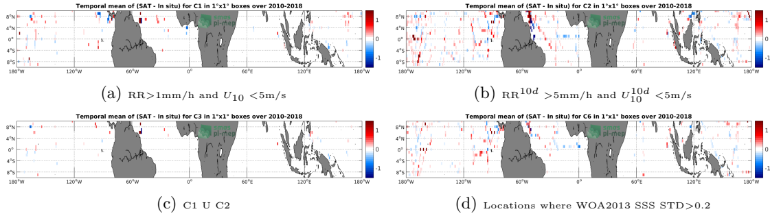
Figure 12: Temporal mean gridded over spatial boxes of size 1^\circ \times 1^\circ of \Delta SSS (SMOS-L3-CATDS-CPDC-V3-MONTHLY-25KM - TSG-SAMOS) for 4 different subdatasets corresponding to: RR>1mm/h and U_{10} < 5\text{m/s} (a), RR^{10d} > 5\text{mm/h} and U_{10}^{10d} < 5\text{m/s} (b), C1 U C2 (c), Locations where WOA2013 SSS STD>0.2 (d).
