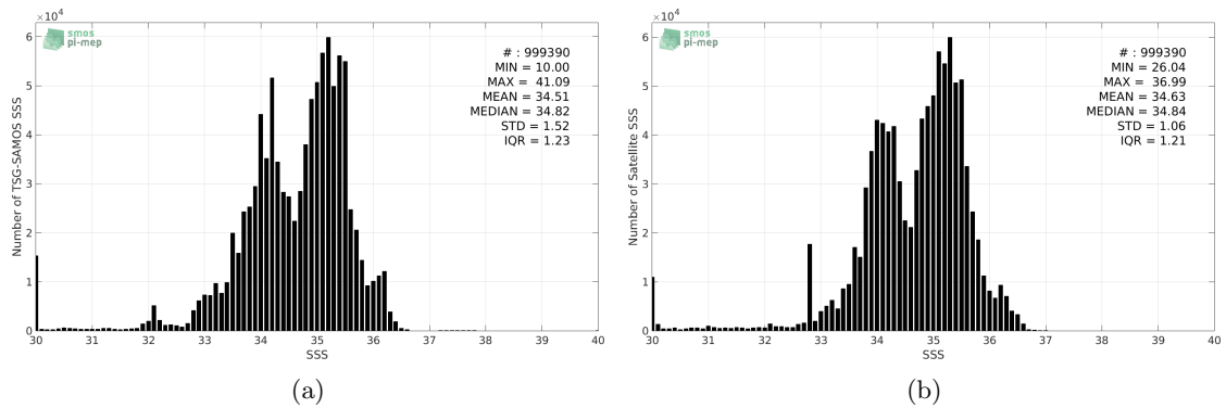
Figure 2: Histograms of SSS from TSG-SAMOS (a) and SMOS-L3-CATDS-CPDC-V3-MONTHLY-25KM (b) considering all match-up pairs per bins of 0.1 over the Equatorial Ocean 10N-10S Pi-MEP region and for the full satellite product period.
