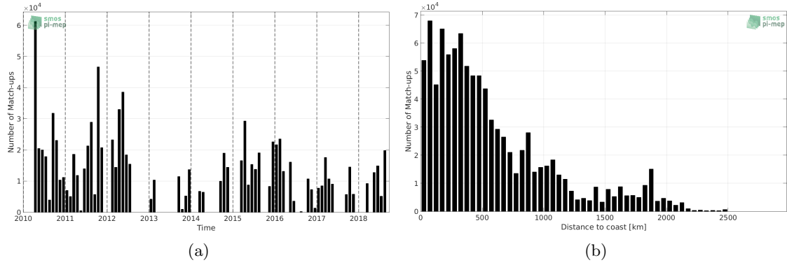
Figure 1: Number of match-ups between TSG-SAMOS and SMOS-L3-CATDS-CPDC-V3-MONTHLY-25KM SSS as a function of time (a) and as function of the distance to coast (b) over the Equatorial Ocean 10N-10S Pi-MEP region and for the full satellite product period.
