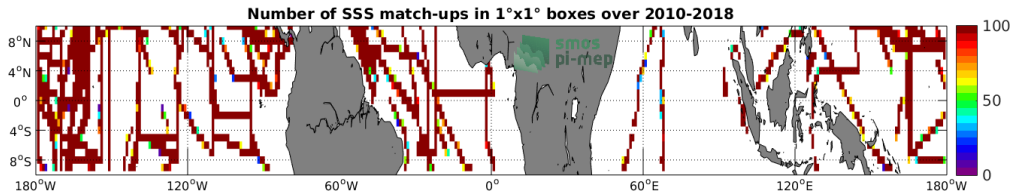
Figure 4: Number of SSS match-ups between TSG-SAMOS SSS and the SMOS-L3-CATDS-CPDC-V3-MONTHLY-25KM SSS product for the Equatorial Ocean 10N-10S Pi-MEP region over 1°x1° boxes and for the full satellite product period.
