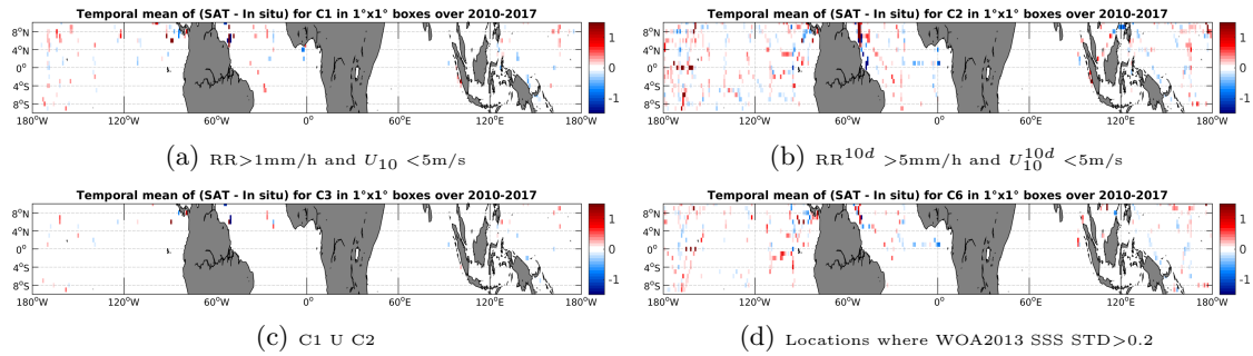
Figure 12: Temporal mean gridded over spatial boxes of size 1^\circ \times 1^\circ of \Delta SSS (SMOS-L3-CATDS-CPDC-V3-MONTHLY-25KM - TSG-SAMOS) for 4 different subdatasets corresponding to: RR > 1\text{mm/h} and U_{10} < 5\text{m/s} (a), RR^{10d} > 5\text{mm/h} and U_{10}^{10d} < 5\text{m/s} (b), C1 U C2 (c), Locations where WOA2013 SSS STD > 0.2 (d).
