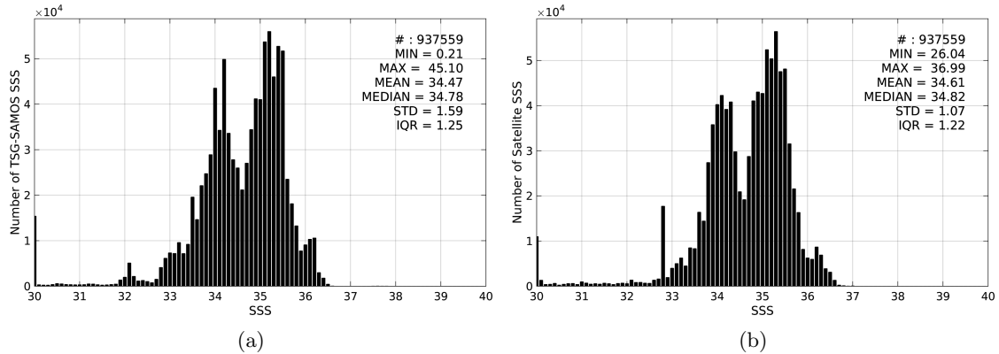
Figure 2: Histograms of SSS from TSG-SAMOS (a) and SMOS-L3-CATDS-CPDC-V3-MONTHLY-25KM (b) considering all match-up pairs per bins of 0.1 over the Equatorial Ocean 10N-10S Pi-MEP region and for the full satellite product period.
