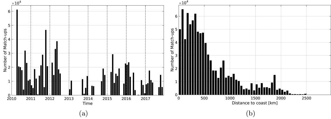
Figure 1: Number of match-ups between TSG-SAMOS and SMOS-L3-CATDS-CPDC-V3-MONTHLY-25KM SSS as a function of time (a) and as function of the distance to coast (b) over the Equatorial Ocean 10N-10S Pi-MEP region and for the full satellite product period.
