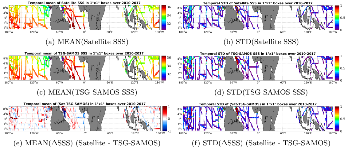
Figure 6: Temporal mean (left) and STD (right) of SSS from SMOS-L3-CATDS-CPDC-V3-MONTHLY-25KM (top), TSG-SAMOS (middle), and of \Delta SSS (Satellite - TSG-SAMOS). Only match-up pairs are used to generate these maps.
