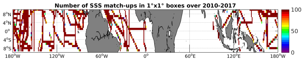
Figure 4: Number of SSS match-ups between TSG-SAMOS SSS and the SMOS-L3-CATDS-CPDC-V3-MONTHLY-25KM SSS product for the Equatorial Ocean 10N-10S Pi-MEP region over 1^\circ \times 1^\circ boxes and for the full satellite product period.
