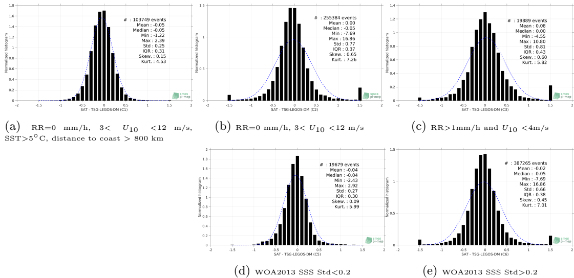
Figure 13: Normalized histogram of ΔSSS (SMOS-L3-CATDS-CPDC-V3-MONTHLY-25KM - TSG-LEGOS-DM) for 5 different subdatasets corresponding to: RR=0 mm/h, 3 < U 10 < 12 m/s, SST>5°C, distance to coast > 800 km (a), RR=0 mm/h, 3 < U 10 < 12 m/s (b), RR>1mm/h and U 10 < 4m/s (c), WOA2013 SSS Std<0.2 (d), WOA2013 SSS Std>0.2 (e).
