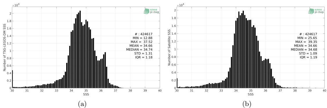
Figure 2: Histograms of SSS from TSG-LEGOS-DM (a) and SMOS-L3-CATDS-CPDC-V3-MONTHLY-25KM (b) considering all match-up pairs per bins of 0.1 over the Equatorial Ocean 10N-10S Pi-MEP region and for the full satellite product period.
