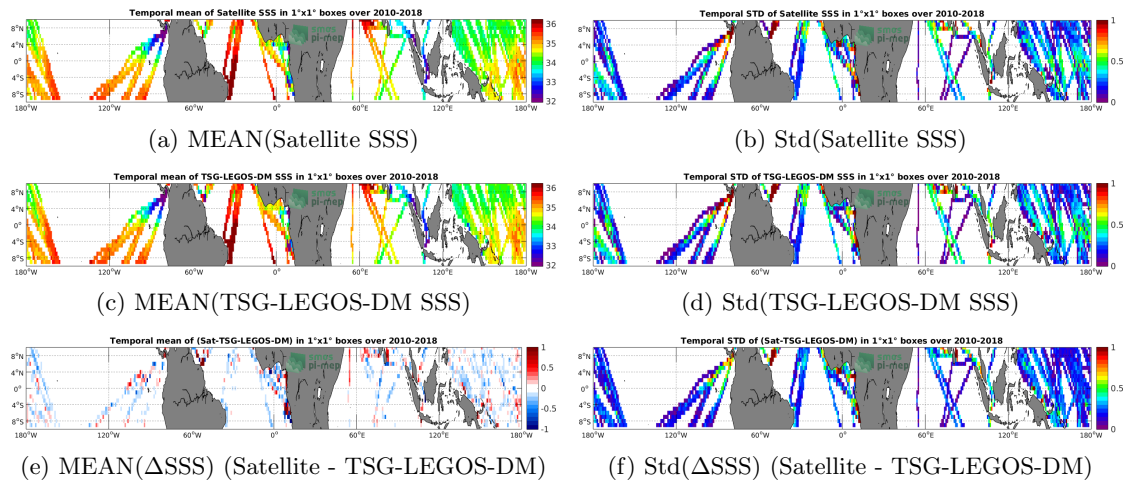
Figure 6: Temporal mean (left) and Std (right) of SSS from SMOS-L3-CATDS-CPDC-V3-MONTHLY-25KM (top), TSG-LEGOS-DM (middle), and of \Delta SSS (Satellite - TSG-LEGOS-DM). Only match-up pairs are used to generate these maps.
