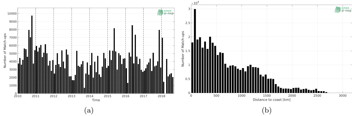
Figure 1: Number of match-ups between TSG-LEGOS-DM and SMOS-L3-CATDS-CPDC-V3-MONTHLY-25KM SSS as a function of time (a) and as function of the distance to coast (b) over the Equatorial Ocean 10N-10S Pi-MEP region and for the full satellite product period.
