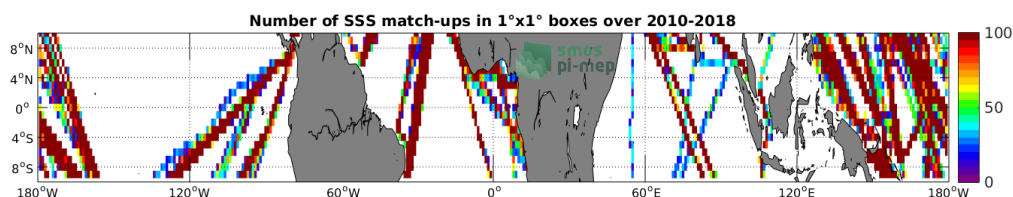
Figure 4: Number of SSS match-ups between TSG-LEGOS-DM SSS and the SMOS-L3-CATDS-CPDC-V3-MONTHLY-25KM SSS product for the Equatorial Ocean 10N-10S Pi-MEP region over 1^\circ \times 1^\circ boxes and for the full satellite product period.
