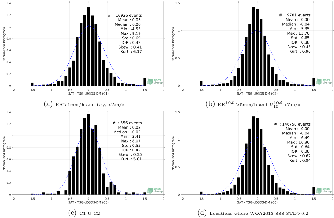
Figure 13: Normalized histogram of \Delta SSS (SMOS-L3-CATDS-CPDC-V3-MONTHLY-25KM - TSG-LEGOS-DM) for 6 different subdatasets corresponding to: RR>1mm/h and U_{10} < 5m/s (a), RR^{10d} > 5mm/h and U_{10}^{10d} < 5m/s (b), C1 U C2 (c), Locations where WOA2013 SSS STD>0.2 (d).
