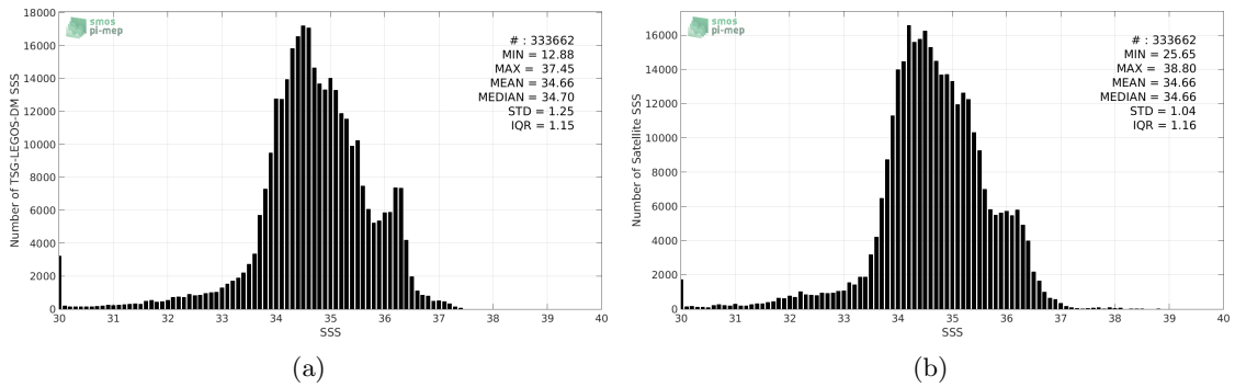
Figure 2: Histograms of SSS from TSG-LEGOS-DM (a) and SMOS-L3-CATDS-CPDC-V3-MONTHLY-25KM (b) considering all match-up pairs per bins of 0.1 over the Equatorial Ocean 10N-10S Pi-MEP region and for the full satellite product period.
