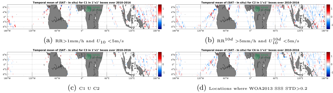
Figure 12: Temporal mean gridded over spatial boxes of size 1^\circ \times 1^\circ of \Delta SSS (SMOS-L3-CATDS-CPDC-V3-MONTHLY-25KM - TSG-LEGOS-DM) for 4 different subdatasets corresponding to: RR>1mm/h and U_{10} < 5m/s (a), RR^{10d} > 5mm/h and U_{10}^{10d} < 5m/s (b), C1 U C2 (c), Locations where WOA2013 SSS STD>0.2 (d).
