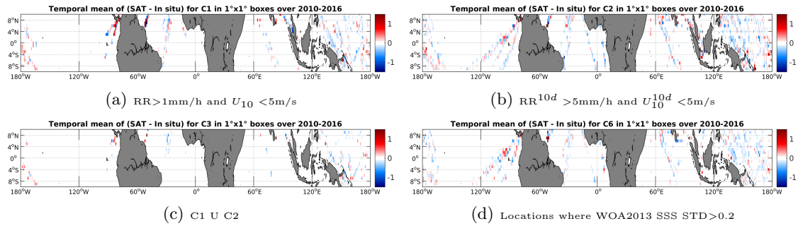
Figure 12: Temporal mean gridded over spatial boxes of size 1^\circ \times 1^\circ of \Delta SSS (SMOS-L3-CATDS-CPDC-V3-MONTHLY-25KM - TSG-LEGOS-DM) for 4 different subdatasets corresponding to: RR > 1\text{mm/h} and U_{10} < 5\text{m/s} (a), RR^{10d} > 5\text{mm/h} and U_{10}^{10d} < 5\text{m/s} (b), C1 U C2 (c), Locations where WOA2013 SSS STD > 0.2 (d).
