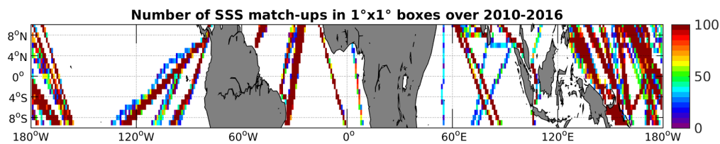
Figure 4: Number of SSS match-ups between TSG-LEGOS-DM SSS and the SMOS-L3-CATDS-CPDC-V3-MONTHLY-25KM SSS product for the Equatorial Ocean 10N-10S Pi-MEP region over 1^\circ \times 1^\circ boxes and for the full satellite product period.
