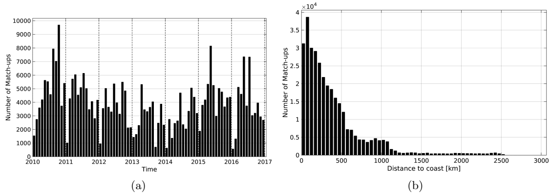
Figure 1: Number of match-ups between TSG-LEGOS-DM and SMOS-L3-CATDS-CPDC-V3-MONTHLY-25KM SSS as a function of time (a) and as function of the distance to coast (b) over the Equatorial Ocean 10N-10S Pi-MEP region and for the full satellite product period.
