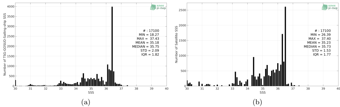
Figure 2: Histograms of SSS from TSG-GOSUD-Sailing-ship (a) and SMOS-L3-CATDS-CPDC-V3-MONTHLY-25KM (b) considering all match-up pairs per bins of 0.1 over the Equatorial Ocean 10N-10S Pi-MEP region and for the full satellite product period.
