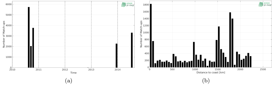
Figure 1: Number of match-ups between TSG-GOSUD-Sailing-ship and SMOS-L3-CATDS-CPDC-V3-MONTHLY-25KM SSS as a function of time (a) and as function of the distance to coast (b) over the Equatorial Ocean 10N-10S Pi-MEP region and for the full satellite product period.
