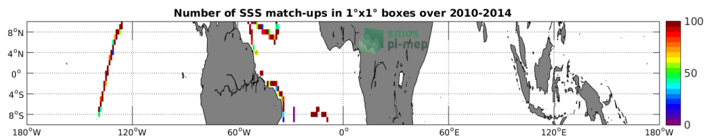
Figure 4: Number of SSS match-ups between TSG-GOSUD-Sailing-ship SSS and the SMOS-L3-CATDS-CPDC-V3-MONTHLY-25KM SSS product for the Equatorial Ocean 10N-10S Pi-MEP region over 1^\circ \times 1^\circ boxes and for the full satellite product period.
