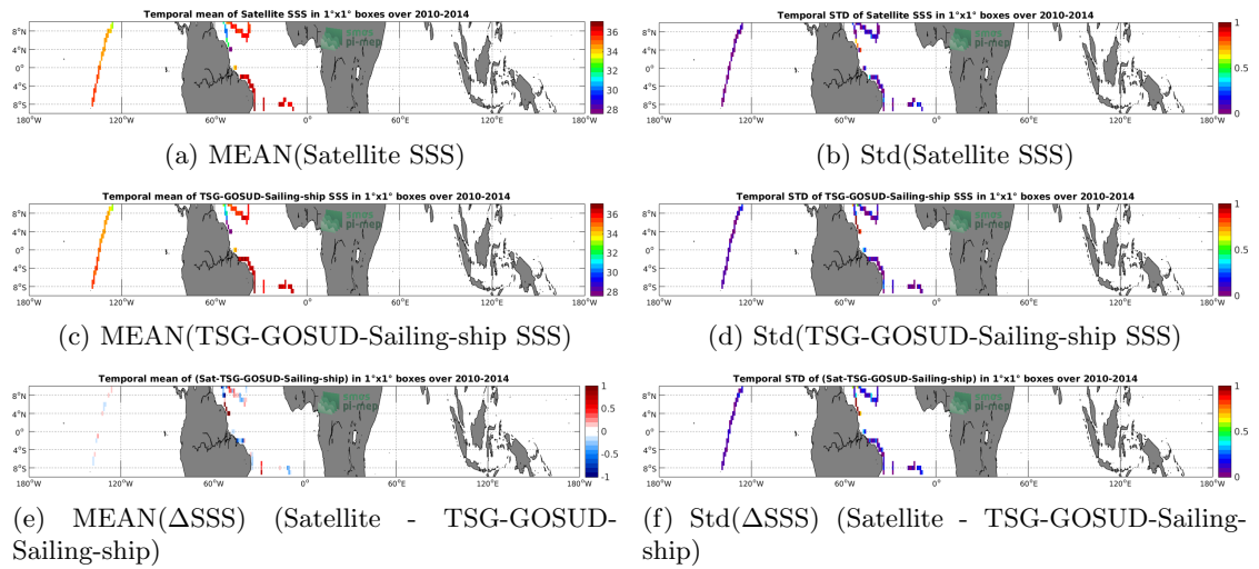
Figure 6: Temporal mean (left) and Std (right) of SSS from SMOS-L3-CATDS-CPDC-V3-MONTHLY-25KM (top), TSG-GOSUD-Sailing-ship (middle), and of \Delta SSS (Satellite - TSG-GOSUD-Sailing-ship). Only match-up pairs are used to generate these maps.
