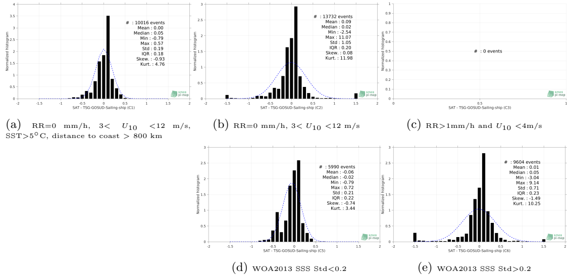
Figure 13: Normalized histogram of \Delta SSS (SMOS-L3-CATDS-CPDC-V3-MONTHLY-25KM - TSG-GOSUD-Sailing-ship) for 5 different subdatasets corresponding to: RR=0 mm/h, 3 < U_{10} < 12 m/s, SST >5^\circ C, distance to coast > 800 km (a), RR=0 mm/h, 3 < U_{10} < 12 m/s (b), RR >1 mm/h and U_{10} < 4 m/s (c), WOA2013 SSS Std <0.2 (d), WOA2013 SSS Std >0.2 (e).
