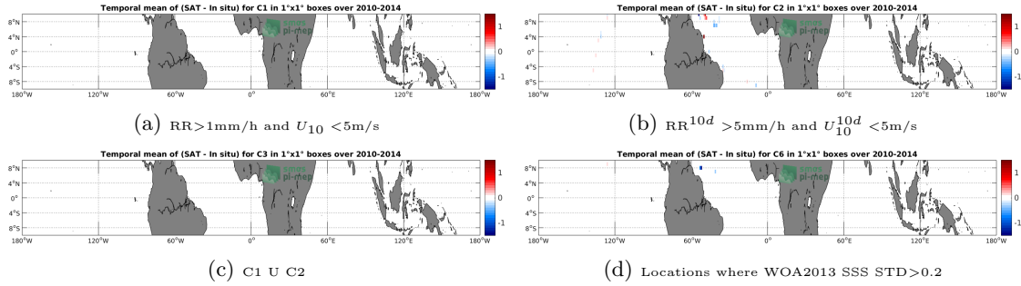
Figure 12: Temporal mean gridded over spatial boxes of size 1^\circ \times 1^\circ of \Delta SSS (SMOS-L3-CATDS-CPDC-V3-MONTHLY-25KM - TSG-GOSUD-Sailing-ship) for 4 different subdatasets corresponding to: RR >1 mm/h and U_{10} < 5 m/s (a), RR ^{10d} > 5 mm/h and U_{10}^{10d} < 5 m/s (b), C1 U C2 (c), Locations where WOA2013 SSS STD >0.2 (d).
