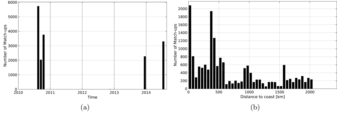
Figure 1: Number of match-ups between TSG-GOSUD-Sailing-ship and SMOS-L3-CATDS-CPDC-V3-MONTHLY-25KM SSS as a function of time (a) and as function of the distance to coast (b) over the Equatorial Ocean 10N-10S Pi-MEP region and for the full satellite product period.
