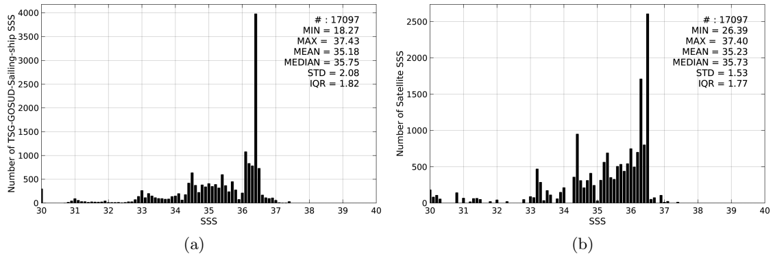
Figure 2: Histograms of SSS from TSG-GOSUD-Sailing-ship (a) and SMOS-L3-CATDS-CPDC-V3-MONTHLY-25KM (b) considering all match-up pairs per bins of 0.1 over the Equatorial Ocean 10N-10S Pi-MEP region and for the full satellite product period.
