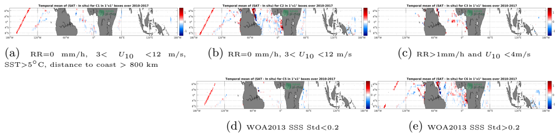
Figure 12: Temporal mean gridded over spatial boxes of size 1^\circ \times 1^\circ of \Delta SSS (SMOS-L3-CATDS-CPDC-V3-MONTHLY-25KM - TSG-GOSUD-Research-vessel) for 5 different subdatasets corresponding to:RR=0 mm/h, 3 < U_{10} < 12 m/s, SST >5^\circ C, distance to coast > 800 km (a), RR=0 mm/h, 3 < U_{10} < 12 m/s (b), RR >1 mm/h and U_{10} < 4 m/s (c), WOA2013 SSS Std <0.2 (d), WOA2013 SSS Std >0.2 (e).
