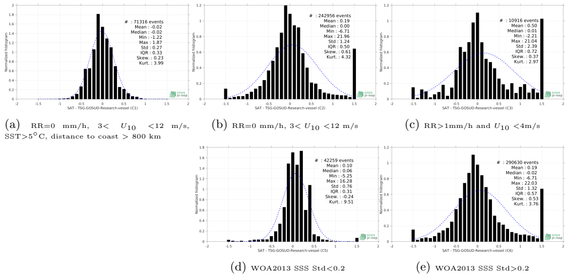
Figure 13: Normalized histogram of \Delta SSS (SMOS-L3-CATDS-CPDC-V3-MONTHLY-25KM - TSG-GOSUD-Research-vessel) for 5 different subdatasets corresponding to: RR=0 mm/h, 3 < U_{10} < 12 m/s, SST >5^\circ C, distance to coast > 800 km (a), RR=0 mm/h, 3 < U_{10} < 12 m/s (b), RR >1 mm/h and U_{10} < 4 m/s (c), WOA2013 SSS Std <0.2 (d), WOA2013 SSS Std >0.2 (e).
