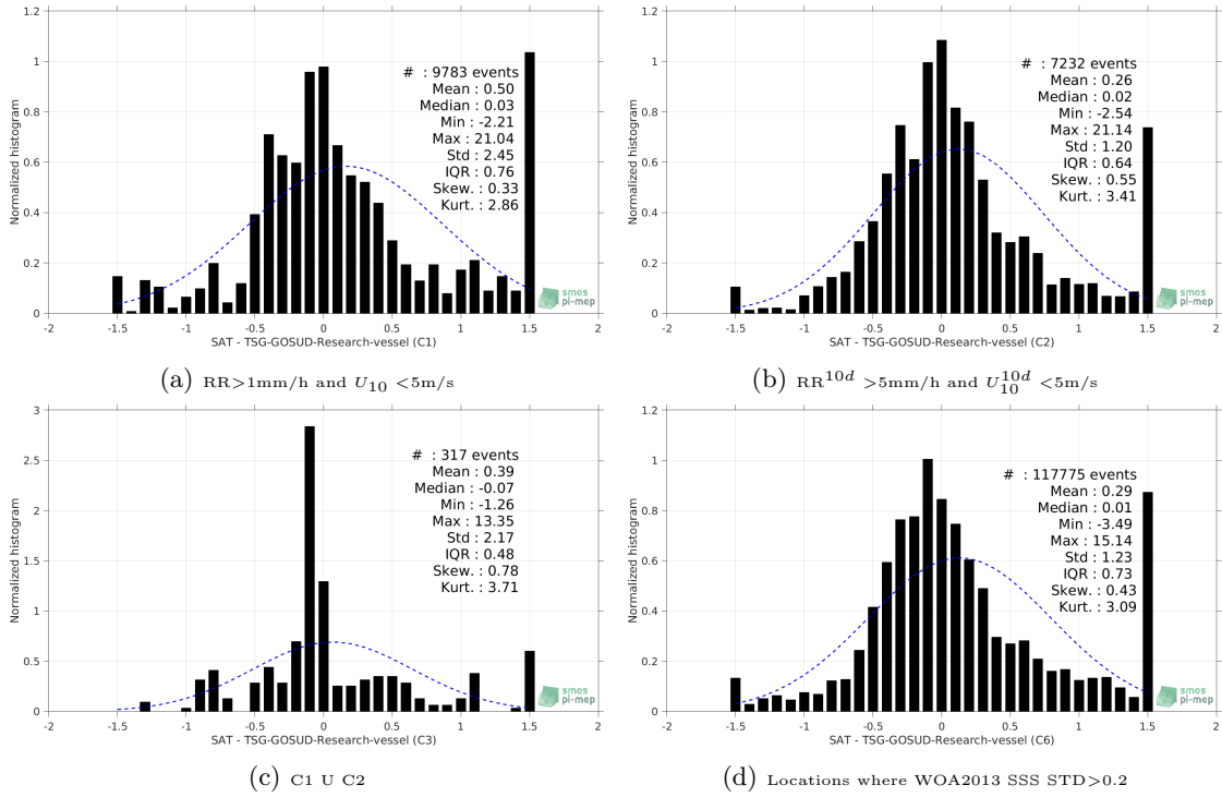
Figure 13: Normalized histogram of \Delta SSS (SMOS-L3-CATDS-CPDC-V3-MONTHLY-25KM - TSG-GOSUD-Research-vessel) for 6 different subdatasets corresponding to: RR>1mm/h and U_{10} < 5\text{m/s} (a), RR^{10d} > 5\text{mm/h} and U_{10}^{10d} < 5\text{m/s} (b), C1 U C2 (c), Locations where WOA2013 SSS STD>0.2 (d).
