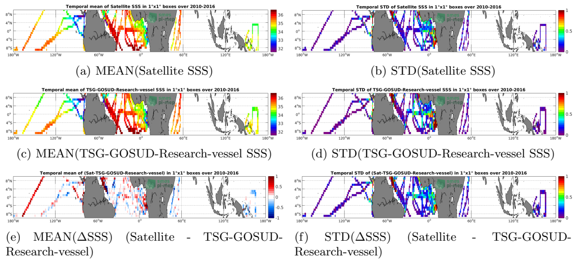
Figure 6: Temporal mean (left) and STD (right) of SSS from SMOS-L3-CATDS-CPDC-V3-MONTHLY-25KM (top), TSG-GOSUD-Research-vessel (middle), and of \Delta SSS (Satellite - TSG-GOSUD-Research-vessel). Only match-up pairs are used to generate these maps.
