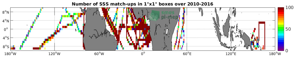
Figure 4: Number of SSS match-ups between TSG-GOSUD-Research-vessel SSS and the SMOS-L3-CATDS-CPDC-V3-MONTHLY-25KM SSS product for the Equatorial Ocean 10N-10S Pi-MEP region over 1°x1° boxes and for the full satellite product period.
