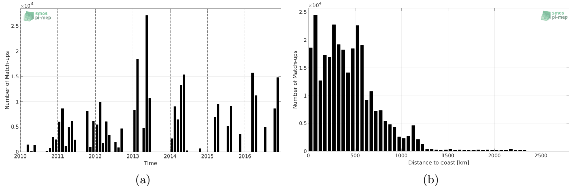
Figure 1: Number of match-ups between TSG-GOSUD-Research-vessel and SMOS-L3-CATDS-CPDC-V3-MONTHLY-25KM SSS as a function of time (a) and as function of the distance to coast (b) over the Equatorial Ocean 10N-10S Pi-MEP region and for the full satellite product period.
