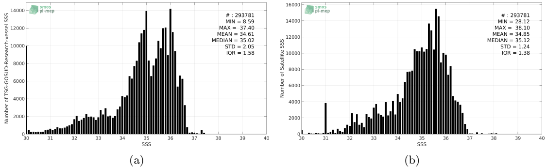
Figure 2: Histograms of SSS from TSG-GOSUD-Research-vessel (a) and SMOS-L3-CATDS-CPDC-V3-MONTHLY-25KM (b) considering all match-up pairs per bins of 0.1 over the Equatorial Ocean 10N-10S Pi-MEP region and for the full satellite product period.
