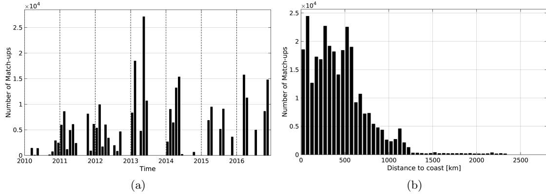
Figure 1: Number of match-ups between TSG-GOSUD-Research-vessel and SMOS-L3-CATDS-CPDC-V3-MONTHLY-25KM SSS as a function of time (a) and as function of the distance to coast (b) over the Equatorial Ocean 10N-10S Pi-MEP region and for the full satellite product period.
