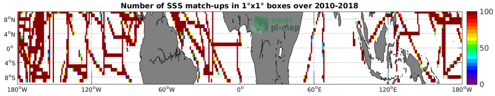
Figure 4: Number of SSS match-ups between TSG-SAMOS SSS and the SMOS-L3-CATDS-CPDC-V3-10DAYS-25KM SSS product for the Equatorial Ocean 10N-10S Pi-MEP region over 1^\circ \times 1^\circ boxes and for the full satellite product period.
