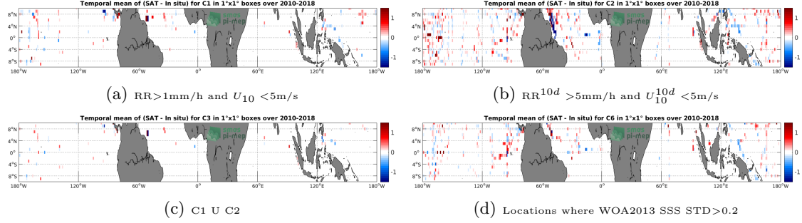
Figure 12: Temporal mean gridded over spatial boxes of size 1^\circ \times 1^\circ of \Delta SSS (SMOS-L3-CATDS-CPDC-V3-10DAYS-25KM - TSG-SAMOS) for 4 different subdatasets corresponding to: RR > 1\text{mm/h} and U_{10} < 5\text{m/s} (a), RR^{10d} > 5\text{mm/h} and U_{10}^{10d} < 5\text{m/s} (b), C1 U C2 (c), Locations where WOA2013 SSS STD > 0.2 (d).
