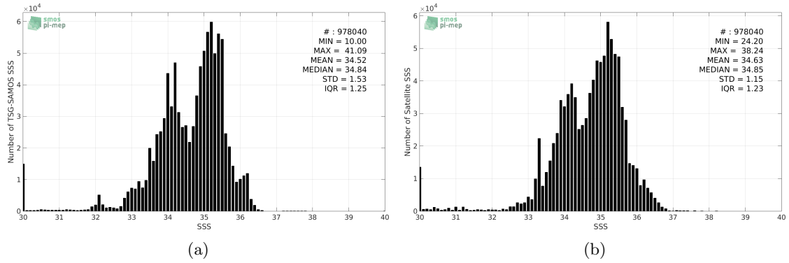
Figure 2: Histograms of SSS from TSG-SAMOS (a) and SMOS-L3-CATDS-CPDC-V3-10DAYS-25KM (b) considering all match-up pairs per bins of 0.1 over the Equatorial Ocean 10N-10S Pi-MEP region and for the full satellite product period.
