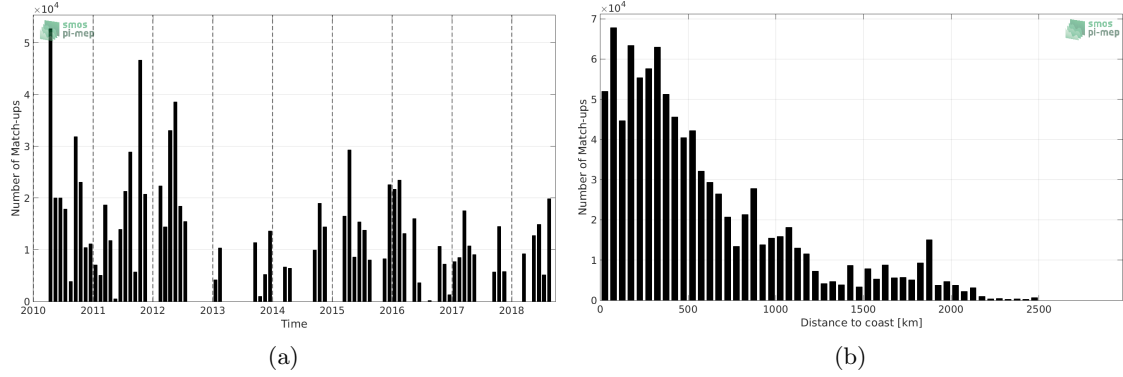
Figure 1: Number of match-ups between TSG-SAMOS and SMOS-L3-CATDS-CPDC-V3-10DAYS-25KM SSS as a function of time (a) and as function of the distance to coast (b) over the Equatorial Ocean 10N-10S Pi-MEP region and for the full satellite product period.
