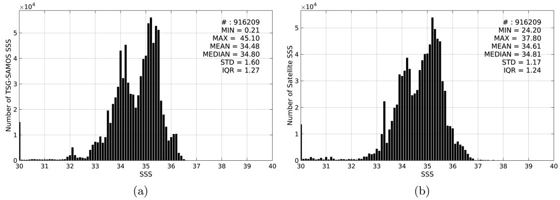
Figure 2: Histograms of SSS from TSG-SAMOS (a) and SMOS-L3-CATDS-CPDC-V3-10DAYS-25KM (b) considering all match-up pairs per bins of 0.1 over the Equatorial Ocean 10N-10S Pi-MEP region and for the full satellite product period.
