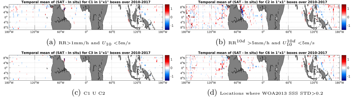
Figure 12: Temporal mean gridded over spatial boxes of size 1^\circ \times 1^\circ of \Delta SSS (SMOS-L3-CATDS-CPDC-V3-10DAYS-25KM - TSG-SAMOS) for 4 different subdatasets corresponding to: RR > 1 mm/h and U_{10} < 5 m/s (a), RR^{10d} > 5 mm/h and U_{10}^{10d} < 5 m/s (b), C1 U C2 (c), Locations where WOA2013 SSS STD > 0.2 (d).
