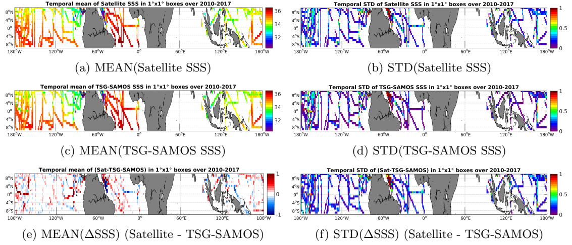
Figure 6: Temporal mean (left) and STD (right) of SSS from SMOS-L3-CATDS-CPDC-V3-10DAYS-25KM (top), TSG-SAMOS (middle), and of \Delta SSS (Satellite - TSG-SAMOS). Only match-up pairs are used to generate these maps.
