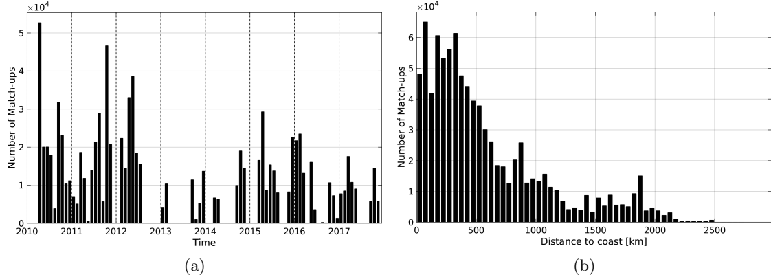
Figure 1: Number of match-ups between TSG-SAMOS and SMOS-L3-CATDS-CPDC-V3-10DAYS-25KM SSS as a function of time (a) and as function of the distance to coast (b) over the Equatorial Ocean 10N-10S Pi-MEP region and for the full satellite product period.
