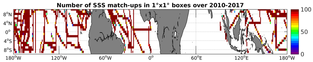
Figure 4: Number of SSS match-ups between TSG-SAMOS SSS and the SMOS-L3-CATDS-CPDC-V3-10DAYS-25KM SSS product for the Equatorial Ocean 10N-10S Pi-MEP region over 1^\circ \times 1^\circ boxes and for the full satellite product period.
