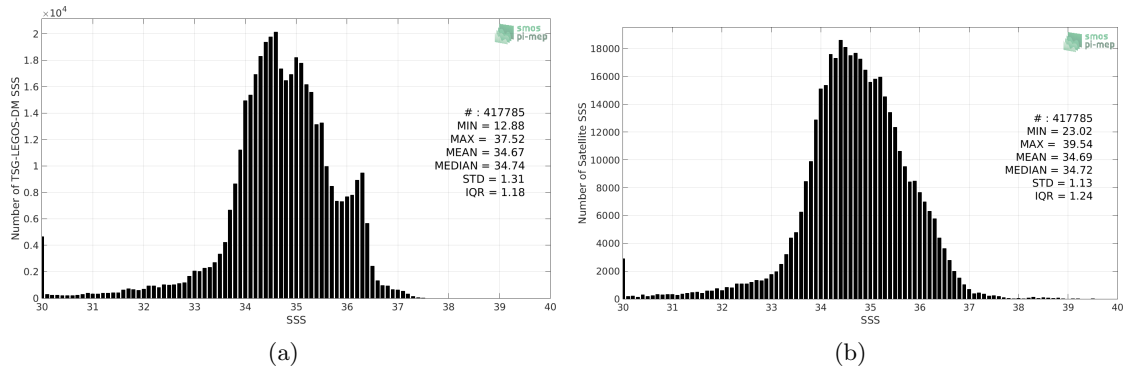
Figure 2: Histograms of SSS from TSG-LEGOS-DM (a) and SMOS-L3-CATDS-CPDC-V3-10DAYS-25KM (b) considering all match-up pairs per bins of 0.1 over the Equatorial Ocean 10N-10S Pi-MEP region and for the full satellite product period.
