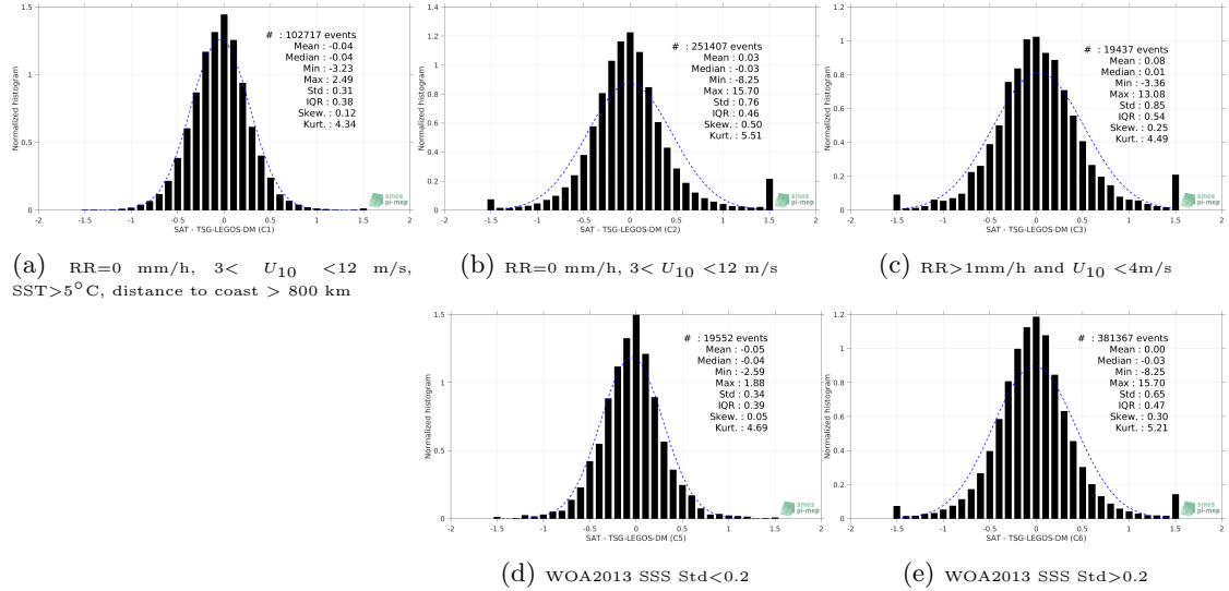
Figure 13: Normalized histogram of \Delta SSS (SMOS-L3-CATDS-CPDC-V3-10DAYS-25KM - TSG-LEGOS-DM) for 5 different subdatasets corresponding to: RR=0 mm/h, 3 < U_{10} < 12 m/s, SST > 5^\circ C , distance to coast > 800 km (a), RR=0 mm/h, 3 < U_{10} < 12 m/s (b), RR > 1 mm/h and U_{10} < 4 m/s (c), WOA2013 SSS Std < 0.2 (d), WOA2013 SSS Std > 0.2 (e).
