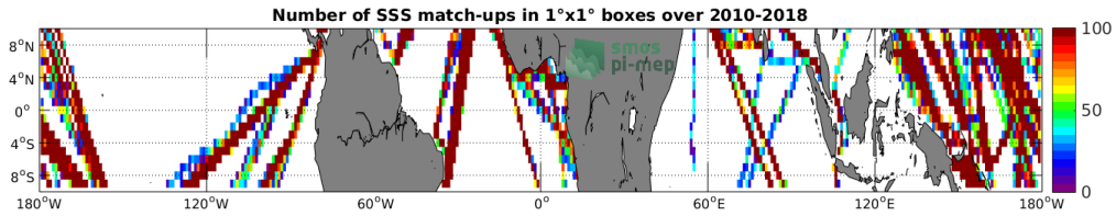
Figure 4: Number of SSS match-ups between TSG-LEGOS-DM SSS and the SMOS-L3-CATDS-CPDC-V3-10DAYS-25KM SSS product for the Equatorial Ocean 10N-10S Pi-MEP region over 1^\circ \times 1^\circ boxes and for the full satellite product period.
