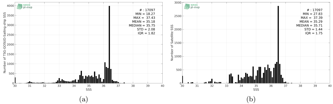
Figure 2: Histograms of SSS from TSG-GOSUD-Sailing-ship (a) and SMOS-L3-CATDS-CPDC-V3-10DAYS-25KM (b) considering all match-up pairs per bins of 0.1 over the Equatorial Ocean 10N-10S Pi-MEP region and for the full satellite product period.
