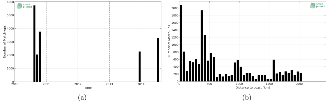
Figure 1: Number of match-ups between TSG-GOSUD-Sailing-ship and SMOS-L3-CATDS-CPDC-V3-10DAYS-25KM SSS as a function of time (a) and as function of the distance to coast (b) over the Equatorial Ocean 10N-10S Pi-MEP region and for the full satellite product period.
