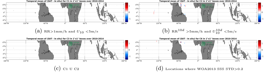
Figure 12: Temporal mean gridded over spatial boxes of size 1^\circ \times 1^\circ of \Delta SSS (SMOS-L3-CATDS-CPDC-V3-10DAYS-25KM - TSG-GOSUD-Sailing-ship) for 4 different subdatasets corresponding to: RR > 1\text{mm/h} and U_{10} < 5\text{m/s} (a), RR^{10d} > 5\text{mm/h} and U_{10}^{10d} < 5\text{m/s} (b), C1 U C2 (c), Locations where WOA2013 SSS STD > 0.2 (d).
