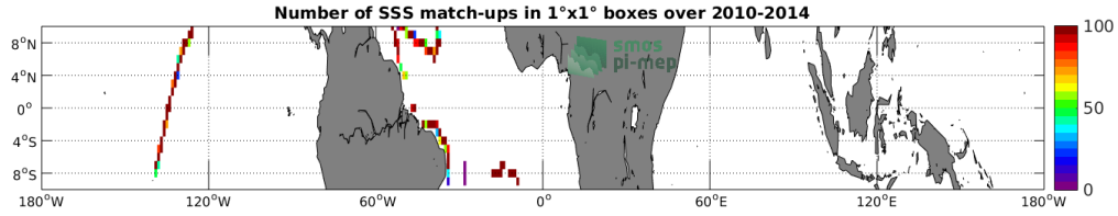
Figure 4: Number of SSS match-ups between TSG-GOSUD-Sailing-ship SSS and the SMOS-L3-CATDS-CPDC-V3-10DAYS-25KM SSS product for the Equatorial Ocean 10N-10S Pi-MEP region over 1°x1° boxes and for the full satellite product period.
