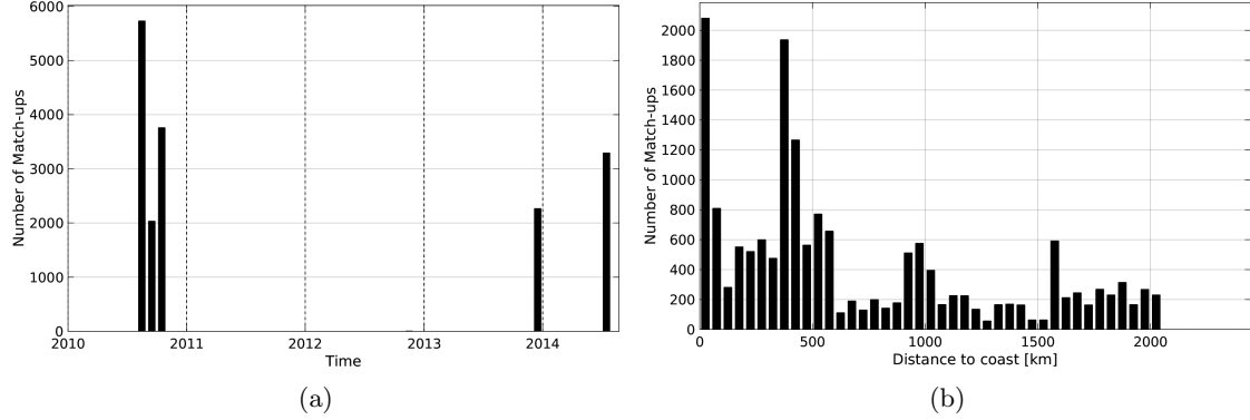
Figure 1: Number of match-ups between TSG-GOSUD-Sailing-ship and SMOS-L3-CATDS-CPDC-V3-10DAYS-25KM SSS as a function of time (a) and as function of the distance to coast (b) over the Equatorial Ocean 10N-10S Pi-MEP region and for the full satellite product period.
