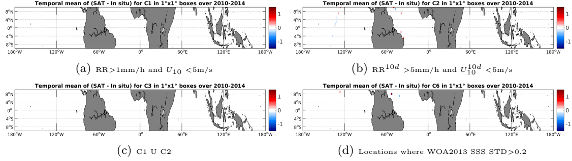
Figure 12: Temporal mean gridded over spatial boxes of size 1^\circ \times 1^\circ of \Delta SSS (SMOS-L3-CATDS-CPDC-V3-10DAYS-25KM - TSG-GOSUD-Sailing-ship) for 4 different subdatasets corresponding to: RR > 1 mm/h and U_{10} < 5 m/s (a), RR ^{10d} > 5 mm/h and U_{10}^{10d} < 5 m/s (b), C1 U C2 (c), Locations where WOA2013 SSS STD > 0.2 (d).
