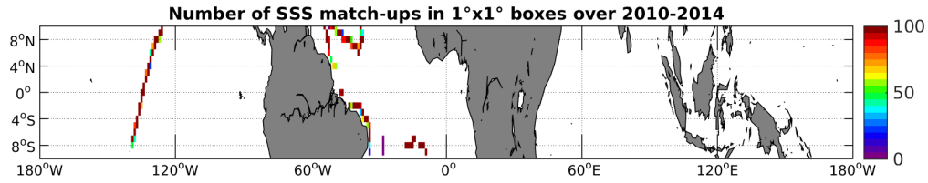
Figure 4: Number of SSS match-ups between TSG-GOSUD-Sailing-ship SSS and the SMOS-L3-CATDS-CPDC-V3-10DAYS-25KM SSS product for the Equatorial Ocean 10N-10S Pi-MEP region over 1°x1° boxes and for the full satellite product period.
