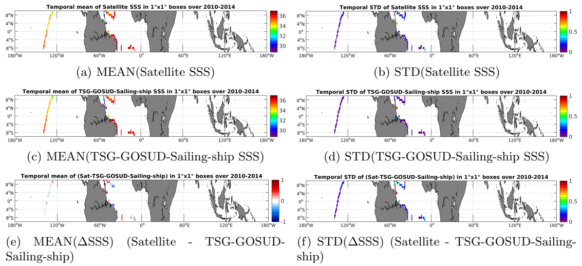
Figure 6: Temporal mean (left) and STD (right) of SSS from SMOS-L3-CATDS-CPDC-V3-10DAYS-25KM (top), TSG-GOSUD-Sailing-ship (middle), and of \Delta SSS (Satellite - TSG-GOSUD-Sailing-ship). Only match-up pairs are used to generate these maps.
