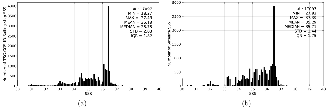
Figure 2: Histograms of SSS from TSG-GOSUD-Sailing-ship (a) and SMOS-L3-CATDS-CPDC-V3-10DAYS-25KM (b) considering all match-up pairs per bins of 0.1 over the Equatorial Ocean 10N-10S Pi-MEP region and for the full satellite product period.
