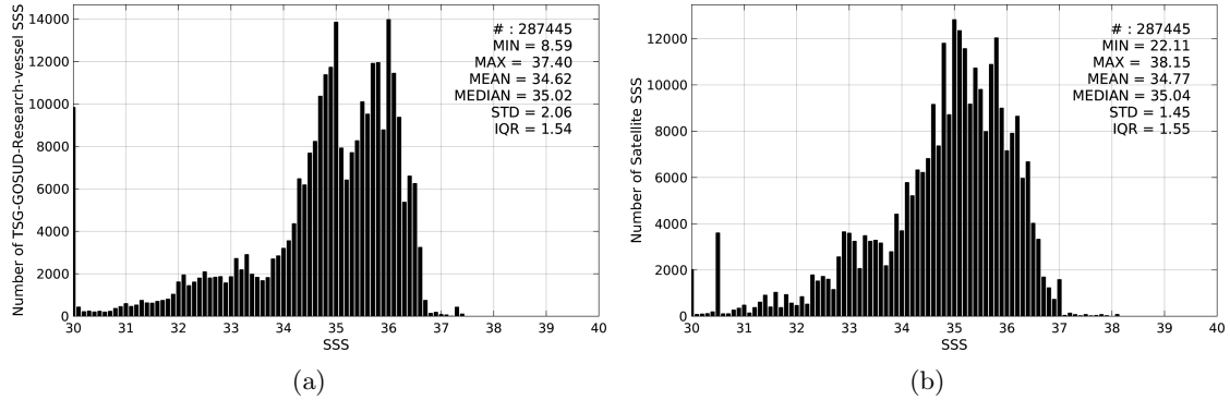
Figure 2: Histograms of SSS from TSG-GOSUD-Research-vessel (a) and SMOS-L3-CATDS-CPDC-V3-10DAYS-25KM (b) considering all match-up pairs per bins of 0.1 over the Equatorial Ocean 10N-10S Pi-MEP region and for the full satellite product period.
