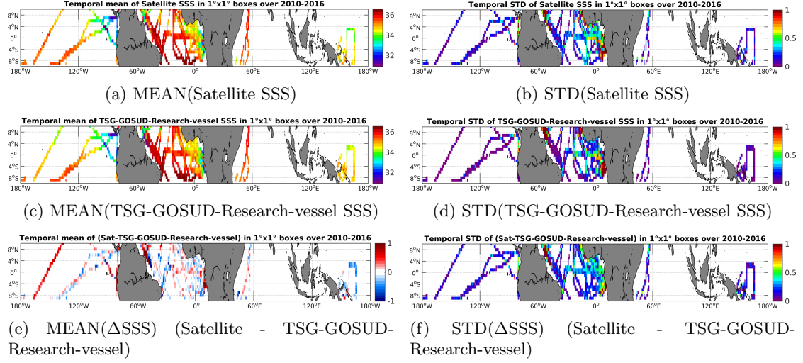
Figure 6: Temporal mean (left) and STD (right) of SSS from SMOS-L3-CATDS-CPDC-V3-10DAYS-25KM (top), TSG-GOSUD-Research-vessel (middle), and of \Delta SSS (Satellite - TSG-GOSUD-Research-vessel). Only match-up pairs are used to generate these maps.
