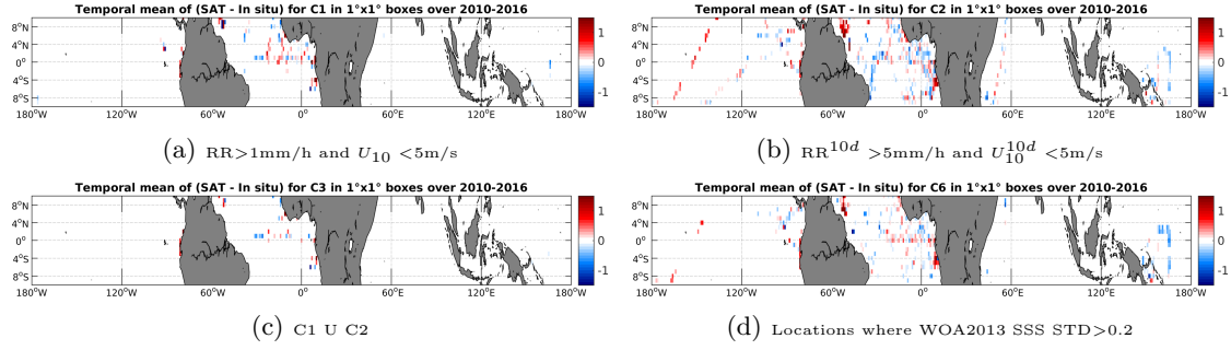
Figure 12: Temporal mean gridded over spatial boxes of size 1^\circ \times 1^\circ of \Delta SSS (SMOS-L3-CATDS-CPDC-V3-10DAYS-25KM - TSG-GOSUD-Research-vessel) for 4 different subdatasets corresponding to: RR > 1mm/h and U_{10} < 5 m/s (a), RR^{10d} > 5 mm/h and U_{10}^{10d} < 5 m/s (b), C1 U C2 (c), Locations where WOA2013 SSS STD > 0.2 (d).
