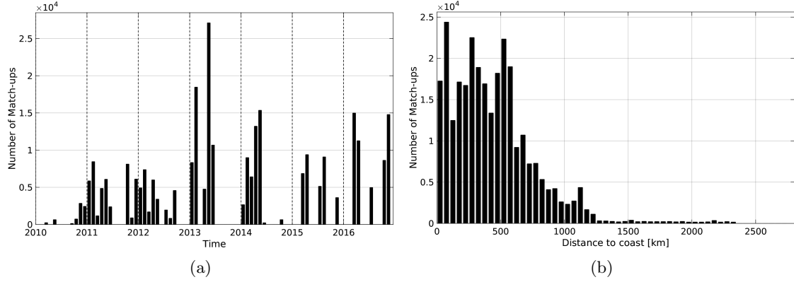
Figure 1: Number of match-ups between TSG-GOSUD-Research-vessel and SMOS-L3-CATDS-CPDC-V3-10DAYS-25KM SSS as a function of time (a) and as function of the distance to coast (b) over the Equatorial Ocean 10N-10S Pi-MEP region and for the full satellite product period.
