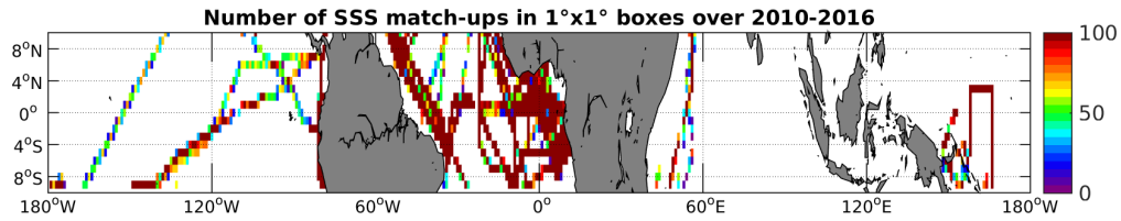
Figure 4: Number of SSS match-ups between TSG-GOSUD-Research-vessel SSS and the SMOS-L3-CATDS-CPDC-V3-10DAYS-25KM SSS product for the Equatorial Ocean 10N-10S Pi-MEP region over 1°x1° boxes and for the full satellite product period.
