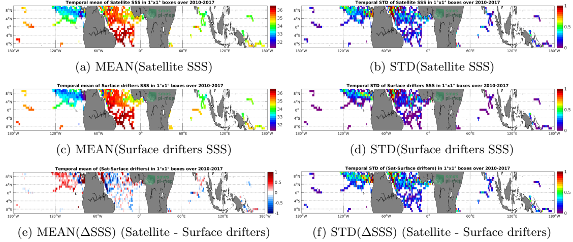
Figure 5: Temporal mean (left) and STD (right) of SSS from SMOS-L3-CATDS-CPDC-V3-10DAYS-25KM (top), Surface drifters (middle), and of \Delta SSS (Satellite - Surface drifters). Only match-up pairs are used to generate these maps.
