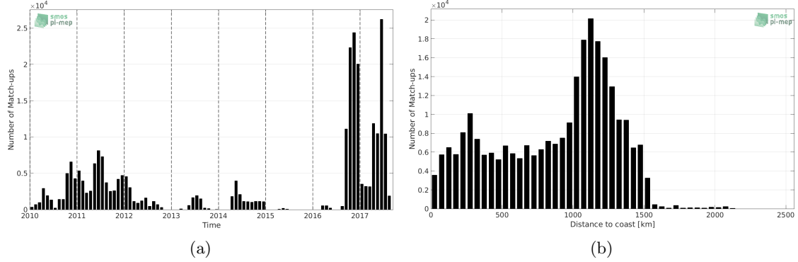
Figure 1: Number of match-ups between Surface drifters and SMOS-L3-CATDS-CPDC-V3-10DAYS-25KM SSS as a function of time (a) and as function of the distance to coast (b) over the Equatorial Ocean 10N-10S Pi-MEP region and for the full satellite product period.
