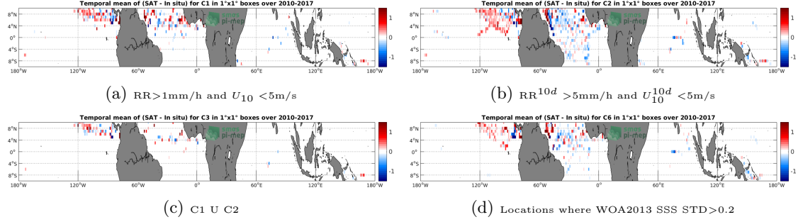
Figure 11: Temporal mean gridded over spatial boxes of size 1^\circ \times 1^\circ of \Delta SSS (SMOS-L3-CATDS-CPDC-V3-10DAYS-25KM - Surface drifters) for 4 different subdatasets corresponding to: RR > 1\text{mm/h} and U_{10} < 5\text{m/s} (a), RR^{10d} > 5\text{mm/h} and U_{10}^{10d} < 5\text{m/s} (b), C1 U C2 (c), Locations where WOA2013 SSS STD > 0.2 (d).
