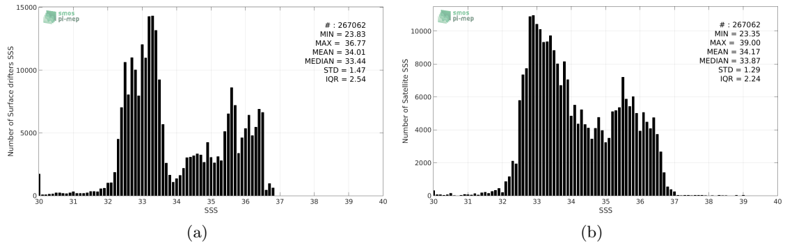
Figure 2: Histograms of SSS from Surface drifters (a) and SMOS-L3-CATDS-CPDC-V3-10DAYS-25KM (b) considering all match-up pairs per bins of 0.1 over the Equatorial Ocean 10N-10S Pi-MEP region and for the full satellite product period.
