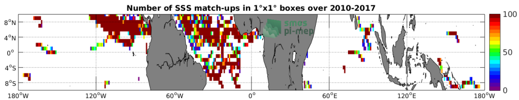
Figure 3: Number of SSS match-ups between Surface drifters SSS and the SMOS-L3-CATDS-CPDC-V3-10DAYS-25KM SSS product for the Equatorial Ocean 10N-10S Pi-MEP region over 1^\circ \times 1^\circ boxes and for the full satellite product period.
