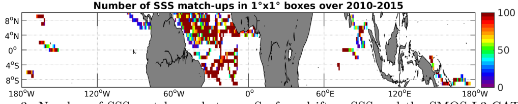
Figure 3: Number of SSS match-ups between Surface drifters SSS and the SMOS-L3-CATDS-CPDC-V3-10DAYS-25KM SSS product for the Equatorial Ocean 10N-10S Pi-MEP region over 1°x1° boxes and for the full satellite product period.
