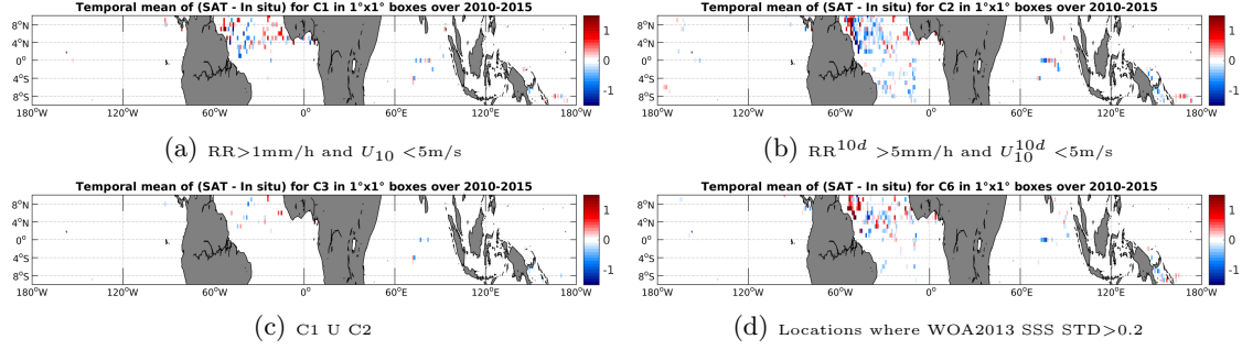
Figure 11: Temporal mean gridded over spatial boxes of size 1^\circ \times 1^\circ of \Delta SSS (SMOS-L3-CATDS-CPDC-V3-10DAYS-25KM - Surface drifters) for 4 different subdatasets corresponding to: RR > 1 mm/h and U_{10} < 5 m/s (a), RR ^{10d} > 5 mm/h and U_{10}^{10d} < 5 m/s (b), C1 U C2 (c), Locations where WOA2013 SSS STD > 0.2 (d).
