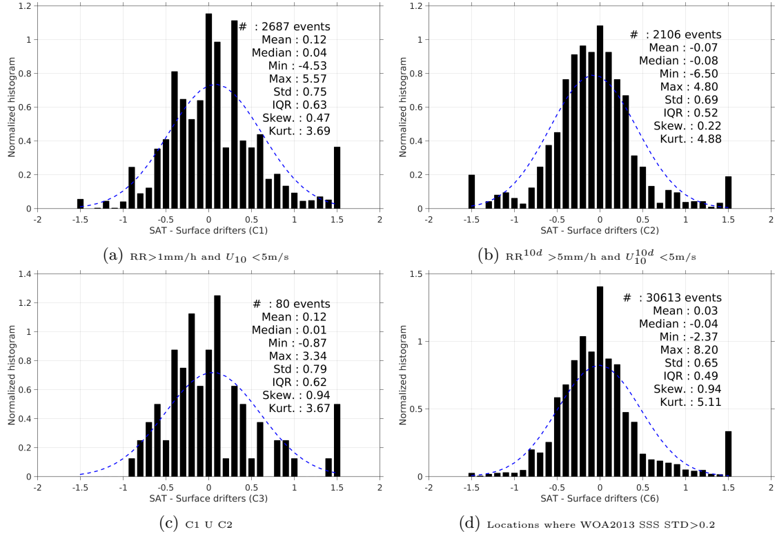
Figure 12: Normalized histogram of \Delta\text{SSS} (SMOS-L3-CATDS-CPDC-V3-10DAYS-25KM - Surface drifters) for 6 different subdatasets corresponding to: \text{RR} > 1\text{mm/h} and U_{10} < 5\text{m/s} (a), \text{RR}^{10d} > 5\text{mm/h} and U_{10}^{10d} < 5\text{m/s} (b), C1 U C2 (c), Locations where WOA2013 SSS STD > 0.2 (d).
