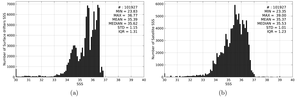
Figure 2: Histograms of SSS from Surface drifters (a) and SMOS-L3-CATDS-CPDC-V3-10DAYS-25KM (b) considering all match-up pairs per bins of 0.1 over the Equatorial Ocean 10N-10S Pi-MEP region and for the full satellite product period.
