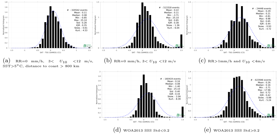
Figure 13: Normalized histogram of \Delta SSS (SMOS SSS L3 v2 - 9-Days (BEC) - TSG (SAMOS)) for 5 different subdatasets corresponding to: RR=0 mm/h, 3 < U_{10} < 12 m/s, SST >5^\circ C, distance to coast > 800 km (a), RR=0 mm/h, 3 < U_{10} < 12 m/s (b), RR >1 mm/h and U_{10} < 4 m/s (c), WOA2013 SSS Std <0.2 (d), WOA2013 SSS Std >0.2 (e).
