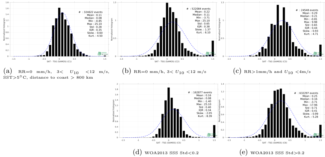
Figure 13: Normalized histogram of \Delta SSS (SMOS SSS L3 v2 - 9-Days (BEC) - TSG (SAMOS)) for 5 different subdatasets corresponding to: RR=0 mm/h, 3 < U_{10} < 12 m/s, SST >5^\circ\text{C} , distance to coast > 800 km (a), RR=0 mm/h, 3 < U_{10} < 12 m/s (b), RR >1 mm/h and U_{10} < 4 m/s (c), WOA2013 SSS Std <0.2 (d), WOA2013 SSS Std >0.2 (e).
