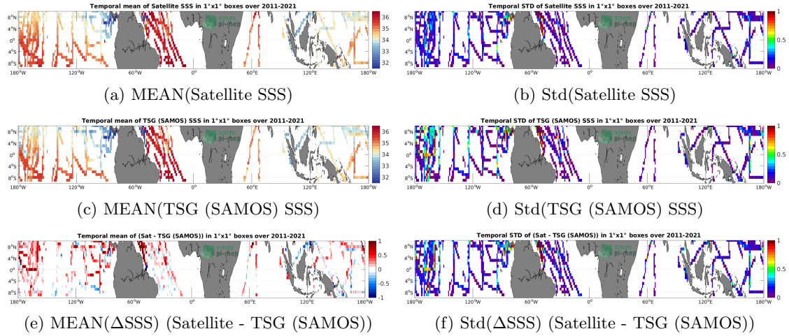
Figure 6: Temporal mean (left) and Std (right) of SSS from SMOS SSS L3 v2 - 9-Days (BEC) (top), TSG (SAMOS) (middle), and of \Delta SSS (Satellite - TSG (SAMOS)). Only match-up pairs are used to generate these maps.
