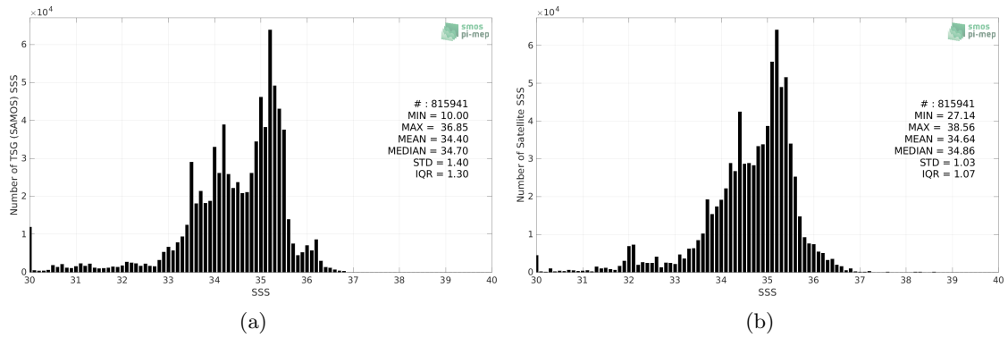
Figure 2: Histograms of SSS from TSG (SAMOS) (a) and SMOS SSS L3 v2 - 9-Days (BEC) (b) considering all match-up pairs per bins of 0.1 over the Equatorial Ocean 10N-10S Pi-MEP region and for the full satellite product period.
