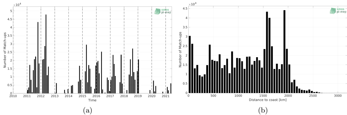
Figure 1: Number of match-ups between TSG (SAMOS) and SMOS SSS L3 v2 - 9-Days (BEC) SSS as a function of time (a) and as function of the distance to coast (b) over the Equatorial Ocean 10N-10S Pi-MEP region and for the full satellite product period.
