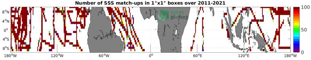
Figure 4: Number of SSS match-ups between TSG (SAMOS) SSS and the SMOS SSS L3 v2 - 9-Days (BEC) SSS product for the Equatorial Ocean 10N-10S Pi-MEP region over 1^\circ \times 1^\circ boxes and for the full satellite product period.
