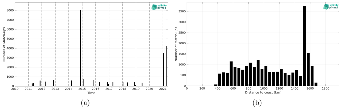
Figure 2: Number of match-ups between TSG (Polarstern) and SMOS SSS L3 v2 - 9-Days (BEC) SSS as a function of time (a) and as function of the distance to coast (b) over the Equatorial Ocean 10N-10S Pi-MEP region and for the full satellite product period.
