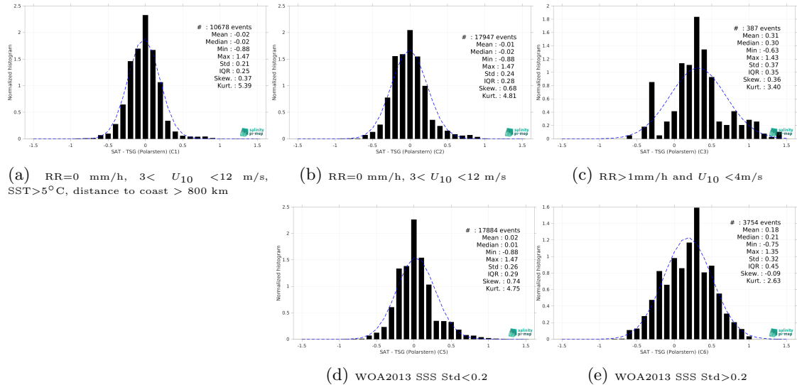
Figure 15: Normalized histogram of \Delta SSS (SMOS SSS L3 v2 - 9-Days (BEC) - TSG (Polarstern)) for 5 different subdatasets corresponding to: RR=0 mm/h, 3 < U_{10} < 12 m/s, SST>5°C, distance to coast > 800 km (a), RR=0 mm/h, 3 < U_{10} < 12 m/s (b), RR>1mm/h and U_{10} < 4 m/s (c), WOA2013 SSS Std<0.2 (d), WOA2013 SSS Std>0.2 (e).
