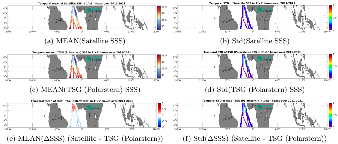
Figure 7: Temporal mean (left) and Std (right) of SSS from SMOS SSS L3 v2 - 9-Days (BEC) (top), TSG (Polarstern) (middle), and of \Delta SSS (Satellite - TSG (Polarstern)). Only match-up pairs are used to generate these maps.
