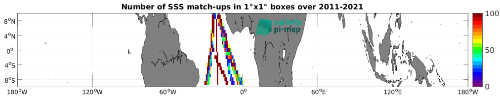
Figure 5: Number of SSS match-ups between TSG (Polarstern) SSS and the SMOS SSS L3 v2 - 9-Days (BEC) SSS product for the Equatorial Ocean 10N-10S Pi-MEP region over 1^\circ \times 1^\circ boxes and for the full satellite product period.
