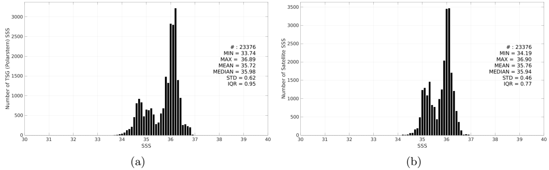
Figure 3: Histograms of SSS from TSG (Polarstern) (a) and SMOS SSS L3 v2 - 9-Days (BEC) (b) considering all match-up pairs per bins of 0.1 over the Equatorial Ocean 10N-10S Pi-MEP region and for the full satellite product period.
