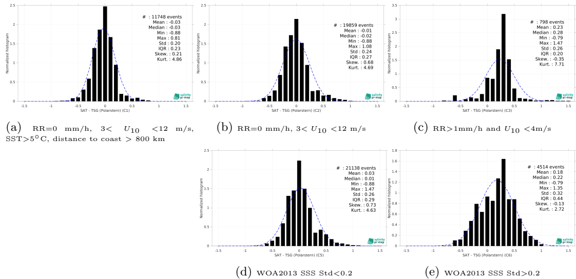
Figure 13: Normalized histogram of \Delta SSS (SMOS SSS L3 v2 - 9-Days (BEC) - TSG (Polarstern)) for 5 different subdatasets corresponding to: RR=0 mm/h, 3 < U_{10} < 12 m/s, SST >5^\circ\text{C} , distance to coast > 800 km (a), RR=0 mm/h, 3 < U_{10} < 12 m/s (b), RR >1 mm/h and U_{10} < 4 m/s (c), WOA2013 SSS Std <0.2 (d), WOA2013 SSS Std >0.2 (e).
