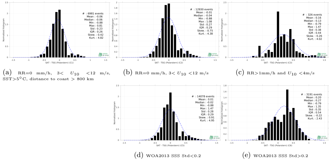
Figure 13: Normalized histogram of \Delta SSS (SMOS SSS L3 v2 - 9-Days (BEC) - TSG (Polarstern)) for 5 different subdatasets corresponding to: RR=0 mm/h, 3 < U_{10} < 12 m/s, SST > 5^\circ C , distance to coast > 800 km (a), RR=0 mm/h, 3 < U_{10} < 12 m/s (b), RR>1mm/h and U_{10} < 4 m/s (c), WOA2013 SSS Std<0.2 (d), WOA2013 SSS Std>0.2 (e).
