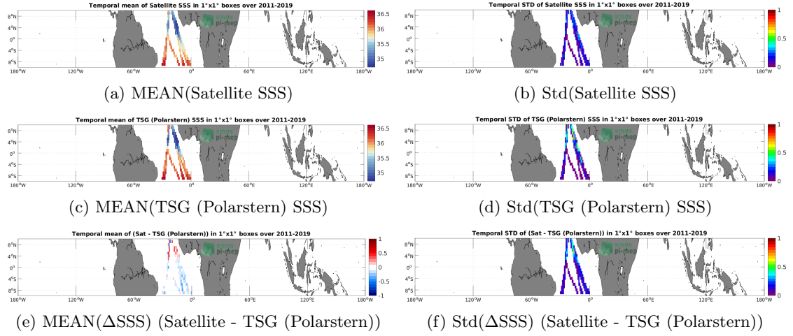
Figure 6: Temporal mean (left) and Std (right) of SSS from SMOS SSS L3 v2 - 9-Days (BEC) (top), TSG (Polarstern) (middle), and of \Delta SSS (Satellite - TSG (Polarstern)). Only match-up pairs are used to generate these maps.
