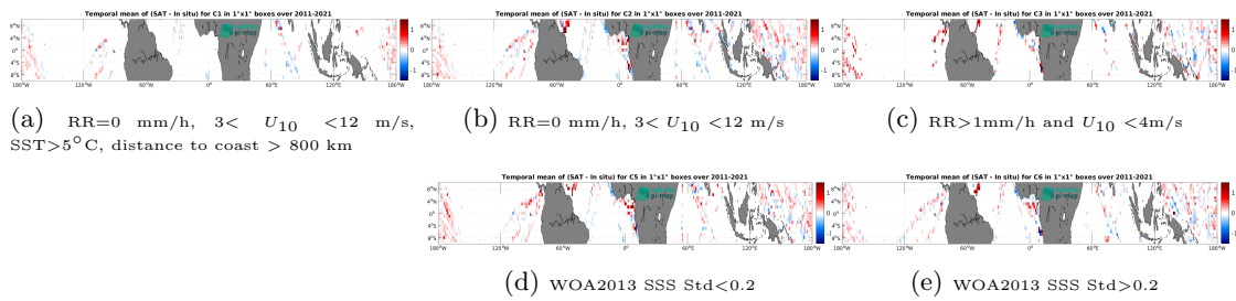
Figure 14: Temporal mean gridded over spatial boxes of size 1^\circ \times 1^\circ of \Delta\text{SSS} (SMOS SSS L3 v2 - 9-Days (BEC) - TSG (LEGOS-DM)) for 5 different subdatasets corresponding to:RR=0 mm/h, 3 < U_{10} < 12 m/s, SST>5°C, distance to coast > 800 km (a), RR=0 mm/h, 3 < U_{10} < 12 m/s (b), RR>1mm/h and U_{10} < 4 m/s (c), WOA2013 SSS Std<0.2 (d), WOA2013 SSS Std>0.2 (e).
