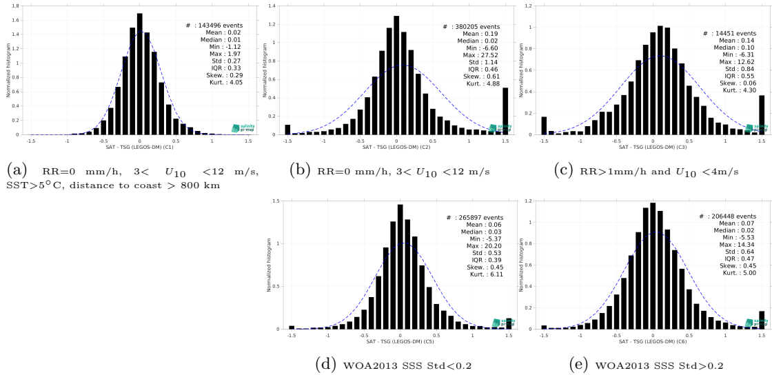
Figure 15: Normalized histogram of \Delta\text{SSS} (SMOS SSS L3 v2 - 9-Days (BEC) - TSG (LEGOS-DM)) for 5 different subdatasets corresponding to: RR=0 mm/h, 3 < U_{10} < 12 m/s, SST>5°C, distance to coast > 800 km (a), RR=0 mm/h, 3 < U_{10} < 12 m/s (b), RR>1mm/h and U_{10} < 4 m/s (c), WOA2013 SSS Std<0.2 (d), WOA2013 SSS Std>0.2 (e).
