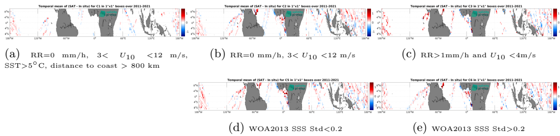
Figure 14: Temporal mean gridded over spatial boxes of size 1^\circ \times 1^\circ of \Delta SSS (SMOS SSS L3 v2 - 9-Days (BEC) - TSG (LEGOS-DM)) for 5 different subdatasets corresponding to:RR=0 mm/h, 3 < U_{10} < 12 m/s, SST>5°C, distance to coast > 800 km (a), RR=0 mm/h, 3 < U_{10} < 12 m/s (b), RR>1mm/h and U_{10} < 4 m/s (c), WOA2013 SSS Std<0.2 (d), WOA2013 SSS Std>0.2 (e).
