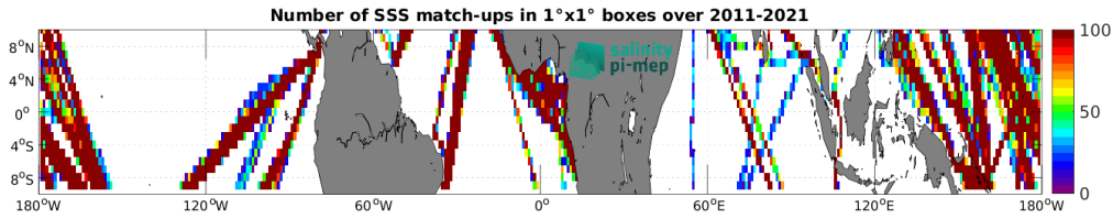
Figure 5: Number of SSS match-ups between TSG (LEGOS-DM) SSS and the SMOS SSS L3 v2 - 9-Days (BEC) SSS product for the Equatorial Ocean 10N-10S Pi-MEP region over 1^\circ \times 1^\circ boxes and for the full satellite product period.
