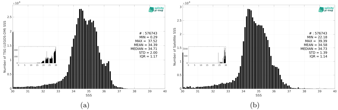
Figure 3: Histograms of SSS from TSG (LEGOS-DM) (a) and SMOS SSS L3 v2 - 9-Days (BEC) (b) considering all match-up pairs per bins of 0.1 over the Equatorial Ocean 10N-10S Pi-MEP region and for the full satellite product period.
