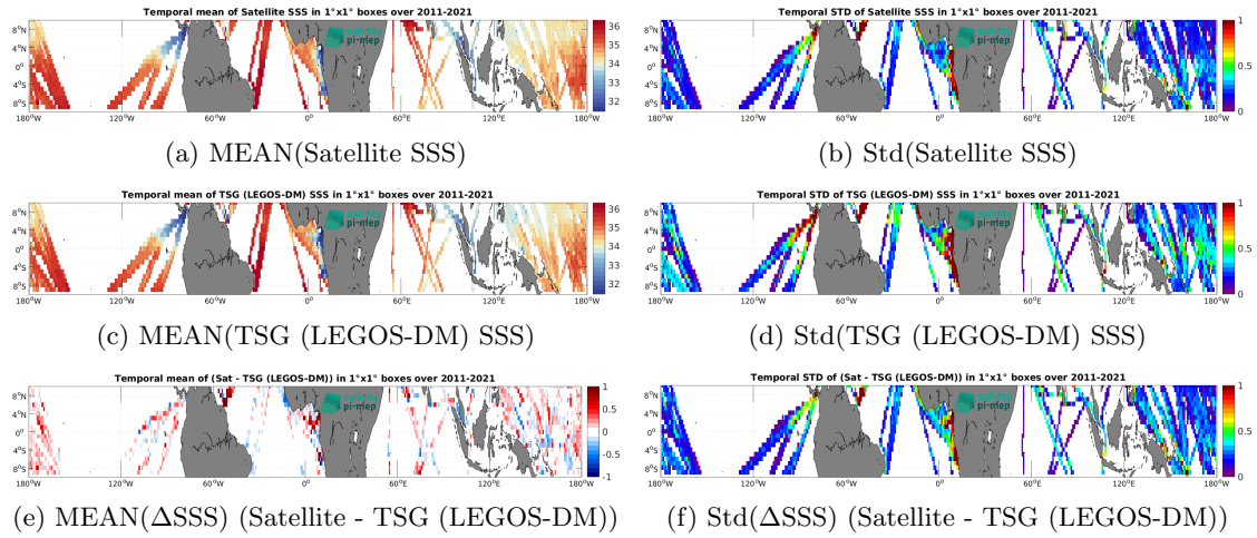
Figure 7: Temporal mean (left) and Std (right) of SSS from SMOS SSS L3 v2 - 9-Days (BEC) (top), TSG (LEGOS-DM) (middle), and of \Delta SSS (Satellite - TSG (LEGOS-DM)). Only match-up pairs are used to generate these maps.
