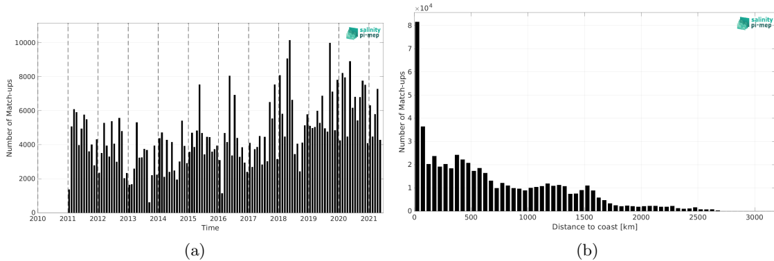
Figure 2: Number of match-ups between TSG (LEGOS-DM) and SMOS SSS L3 v2 - 9-Days (BEC) SSS as a function of time (a) and as function of the distance to coast (b) over the Equatorial Ocean 10N-10S Pi-MEP region and for the full satellite product period.
