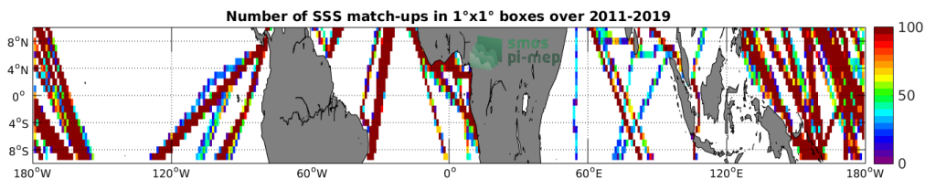
Figure 4: Number of SSS match-ups between TSG (LEGOS-DM) SSS and the SMOS L3 v2 - 9-Days (BEC) SSS product for the Equatorial Ocean 10N-10S Pi-MEP region over 1°x1° boxes and for the full satellite product period.
