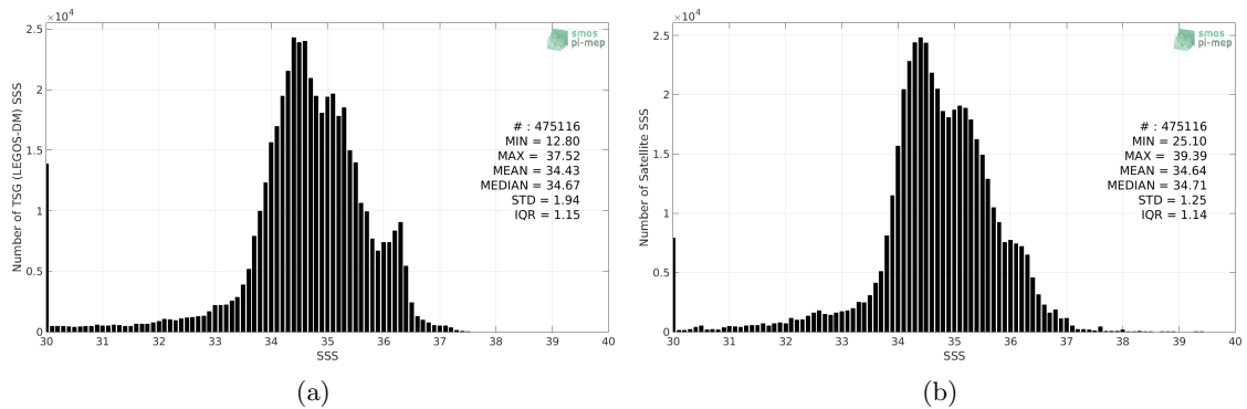
Figure 2: Histograms of SSS from TSG (LEGOS-DM) (a) and SMOS L3 v2 - 9-Days (BEC) (b) considering all match-up pairs per bins of 0.1 over the Equatorial Ocean 10N-10S Pi-MEP region and for the full satellite product period.
