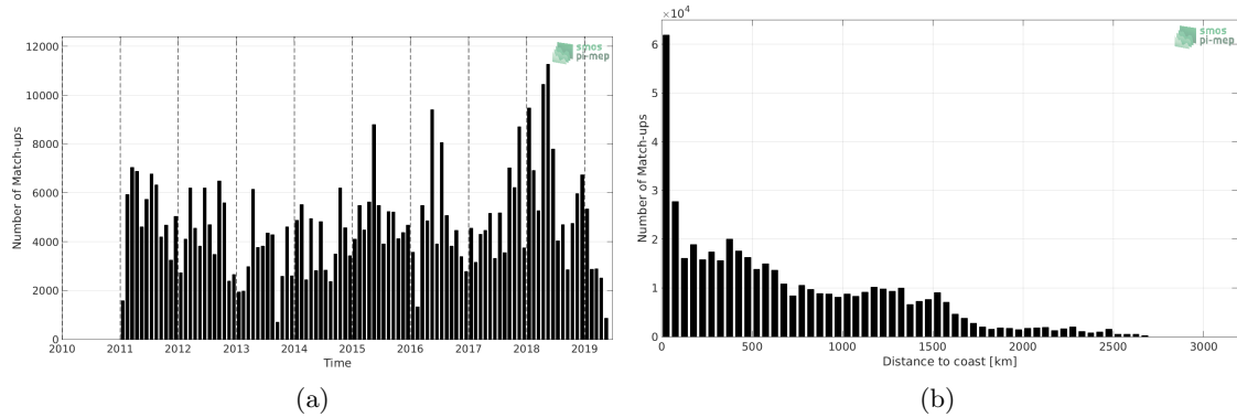
Figure 1: Number of match-ups between TSG (LEGOS-DM) and SMOS L3 v2 - 9-Days (BEC) SSS as a function of time (a) and as function of the distance to coast (b) over the Equatorial Ocean 10N-10S Pi-MEP region and for the full satellite product period.
