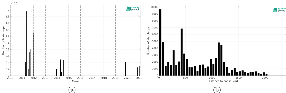
Figure 2: Number of match-ups between TSG (GOSUD-Sailing-ship) and SMOS SSS L3 v2 - 9-Days (BEC) SSS as a function of time (a) and as function of the distance to coast (b) over the Equatorial Ocean 10N-10S Pi-MEP region and for the full satellite product period.
