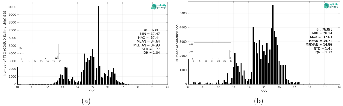
Figure 3: Histograms of SSS from TSG (GOSUD-Sailing-ship) (a) and SMOS SSS L3 v2 - 9-Days (BEC) (b) considering all match-up pairs per bins of 0.1 over the Equatorial Ocean 10N-10S Pi-MEP region and for the full satellite product period.
