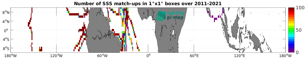
Figure 5: Number of SSS match-ups between TSG (GOSUD-Sailing-ship) SSS and the SMOS SSS L3 v2 - 9-Days (BEC) SSS product for the Equatorial Ocean 10N-10S Pi-MEP region over 1^\circ \times 1^\circ boxes and for the full satellite product period.
