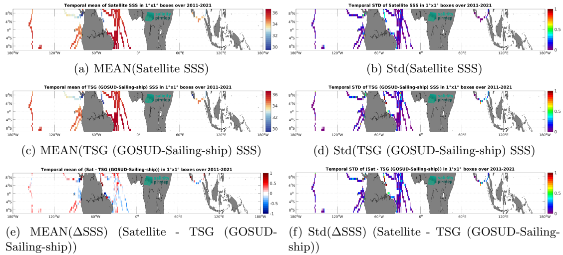
Figure 7: Temporal mean (left) and Std (right) of SSS from SMOS SSS L3 v2 - 9-Days (BEC) (top), TSG (GOSUD-Sailing-ship) (middle), and of \Delta SSS (Satellite - TSG (GOSUD-Sailing-ship)). Only match-up pairs are used to generate these maps.
